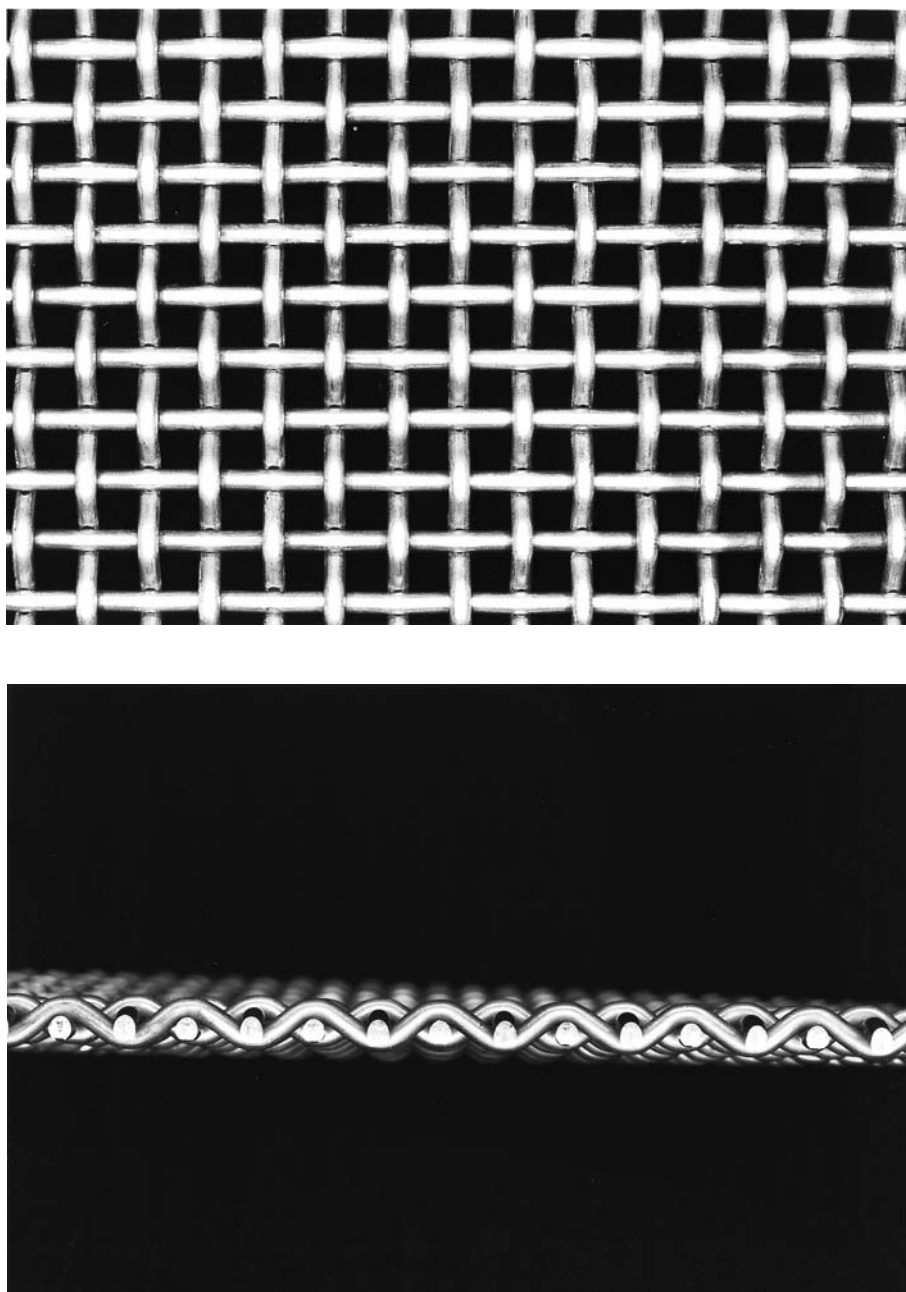
FIG. 5 Double Crimp
