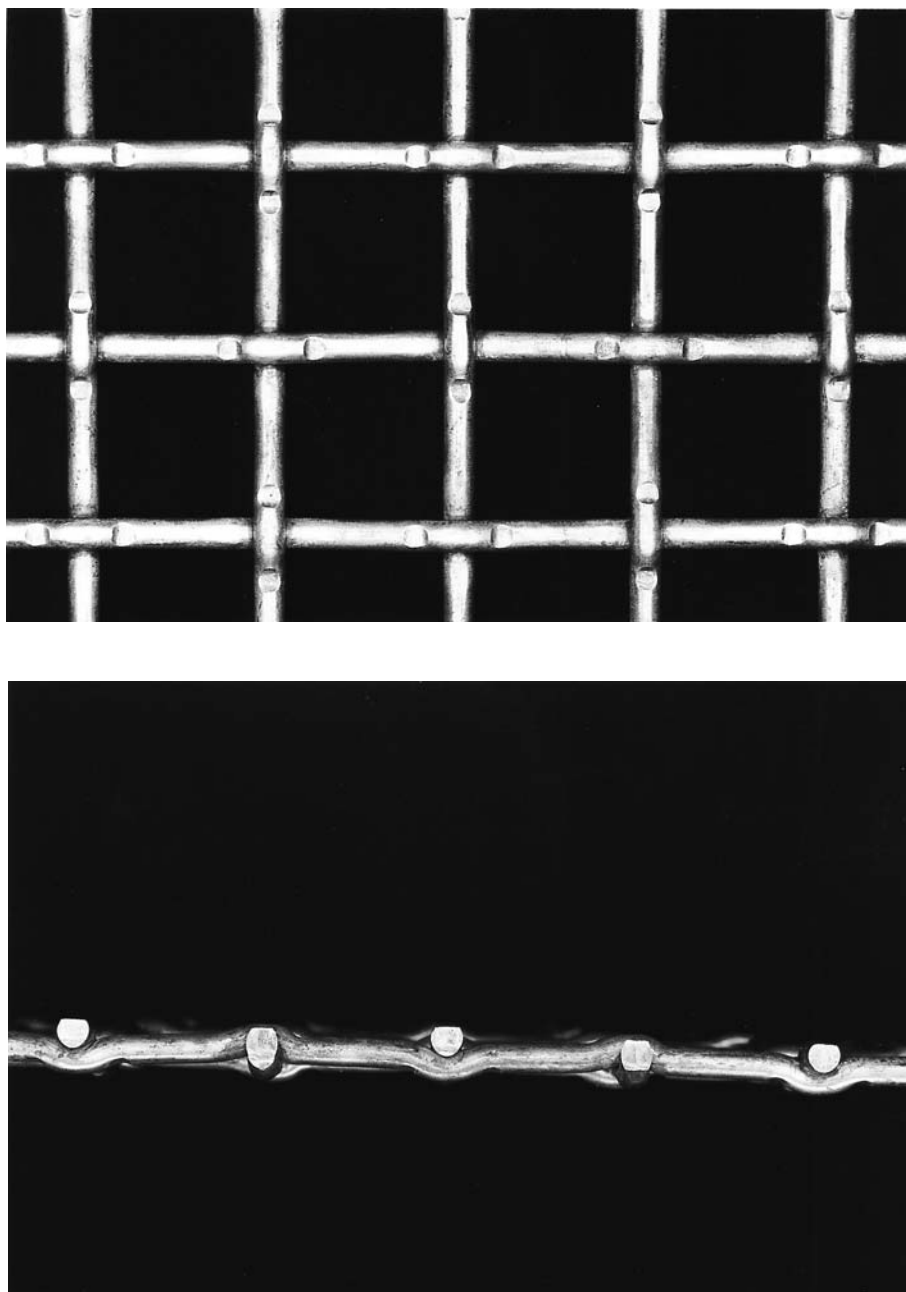
FIG. 8 Lock Crimp
