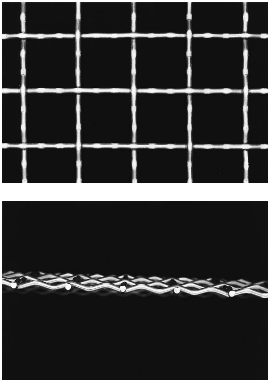
FIG. 7 Intermediate Crimp
