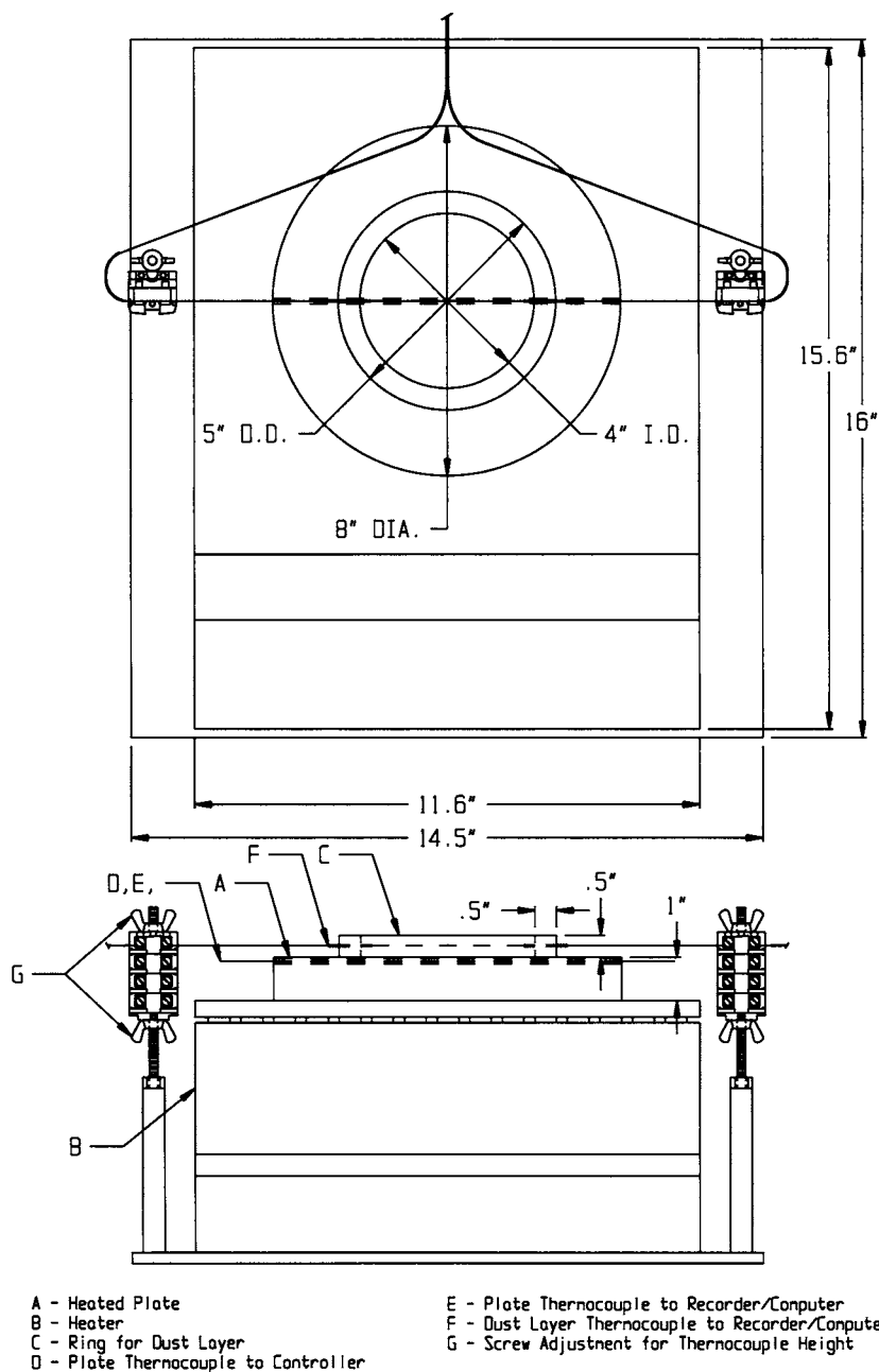
FIG. X2.2 Top View and Side View of Hot-Surface Layer Ignition Apparatus
