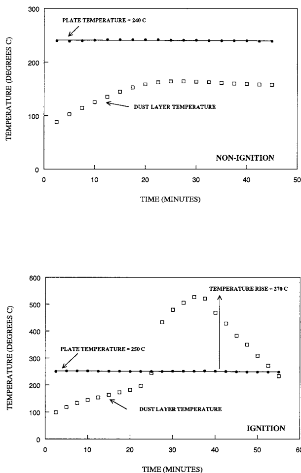
FIG. X3.1 Examples of Hotplate Layer Ignition Test Data
