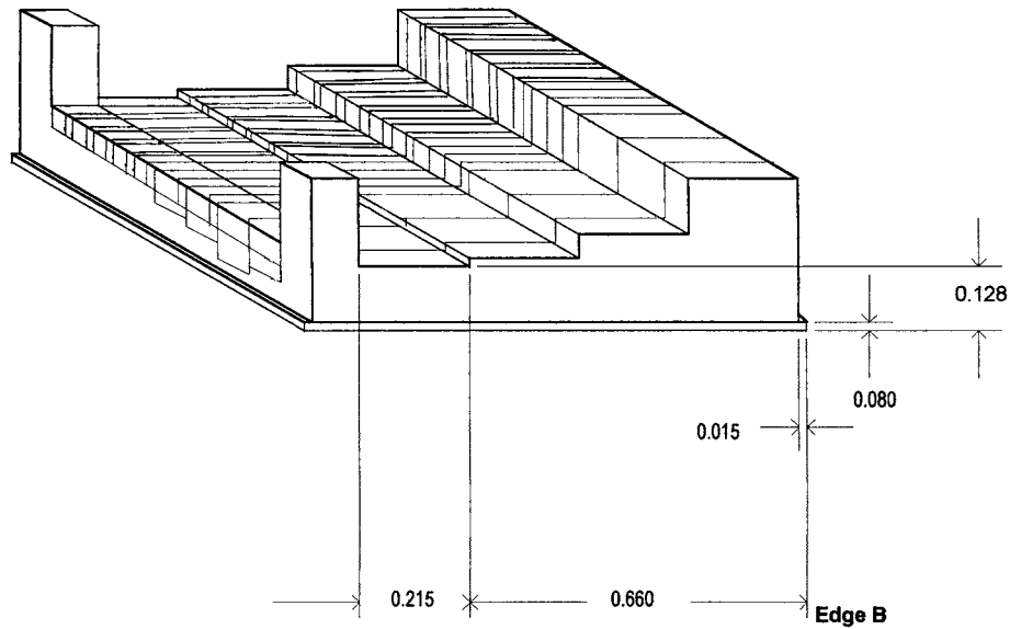
FIG. 8 Second Milled Step
