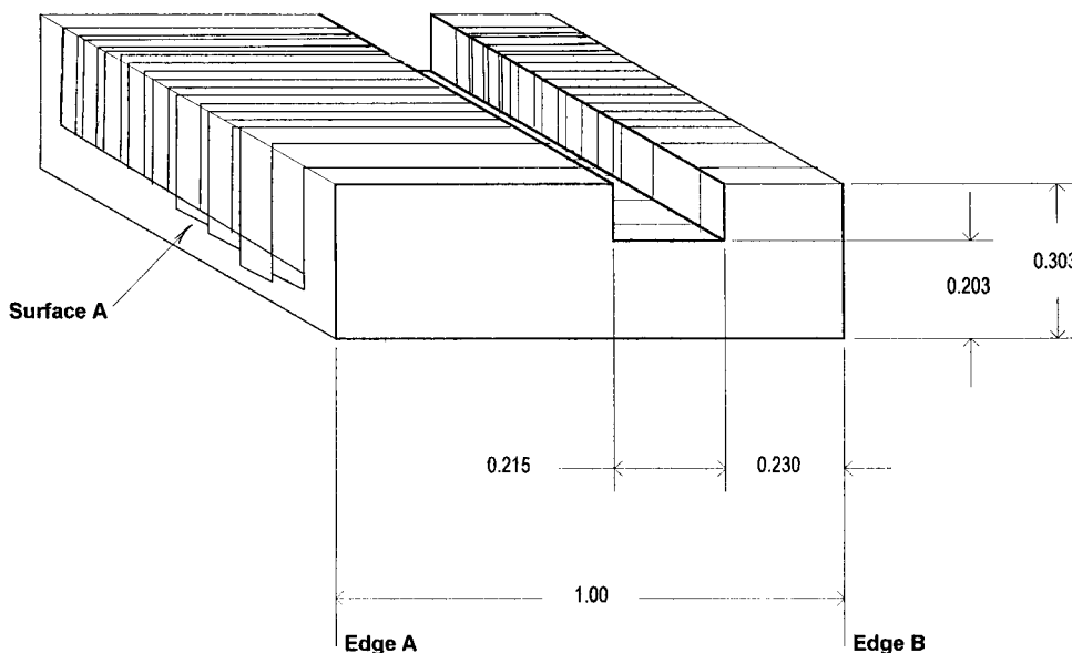
FIG. 7 First Milled Step
