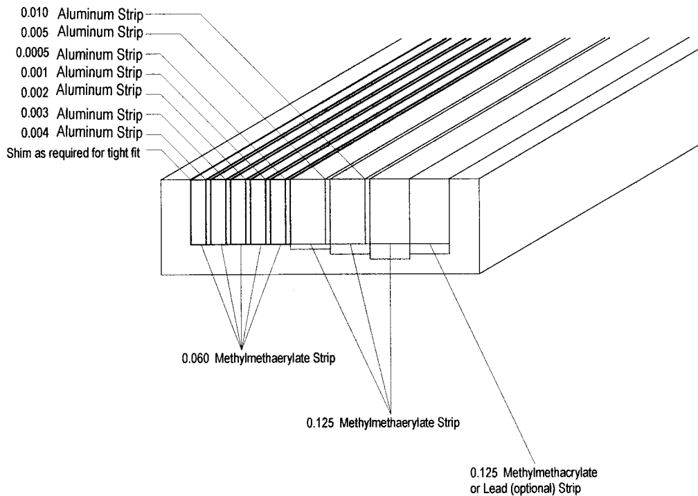
NOTE 1—See Fig. 4. FIG. 5 Shims in Channels
