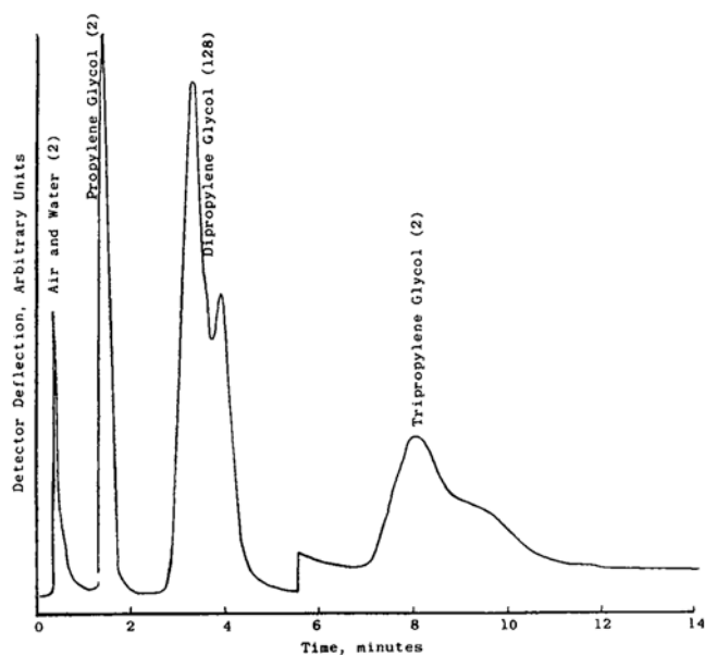
FIG. X2.5 Chromatogram of Dipropylene Glycol Isothermal Operation at 190°C (Recorder Attenuation in Parentheses)
