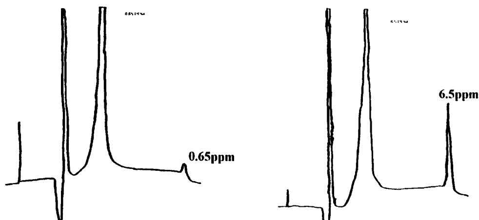
FIG. 3 Typical Chromatograms
