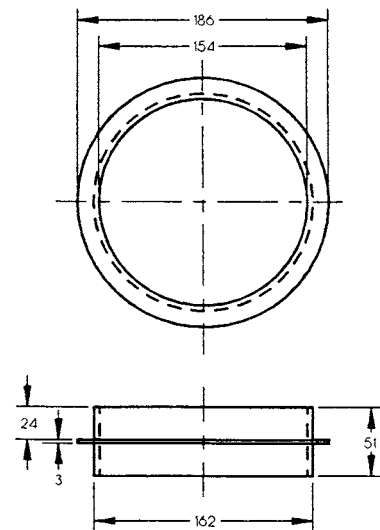
STAINLESS STEEL CONNECTOR ALL DIMENSIONS ARE mm UNLESS NOTED
