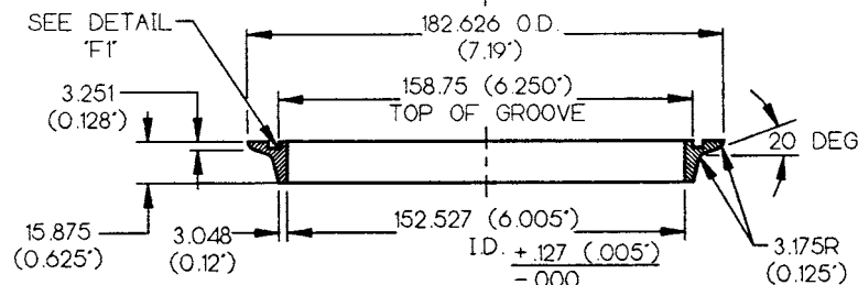
FIG. 13 Duct Flanges
