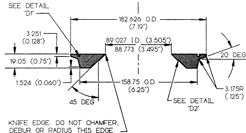
FIG. 10 Funnel Flange
