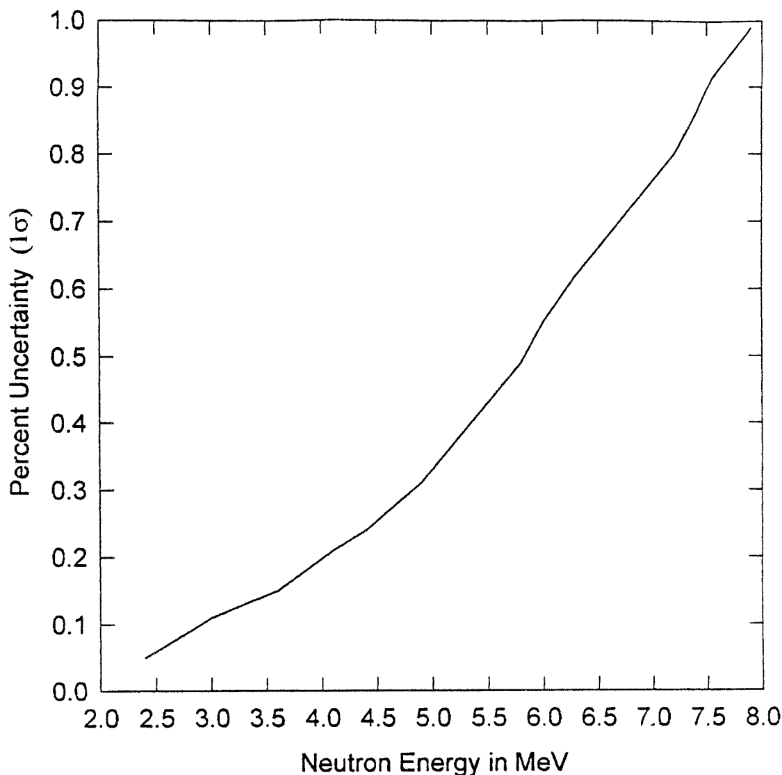
FIG. 11 Uncertainty Introduced into Neutron Fluence by Finite Size Correction for Proton-Recoil Escape from a 400μ NRE
