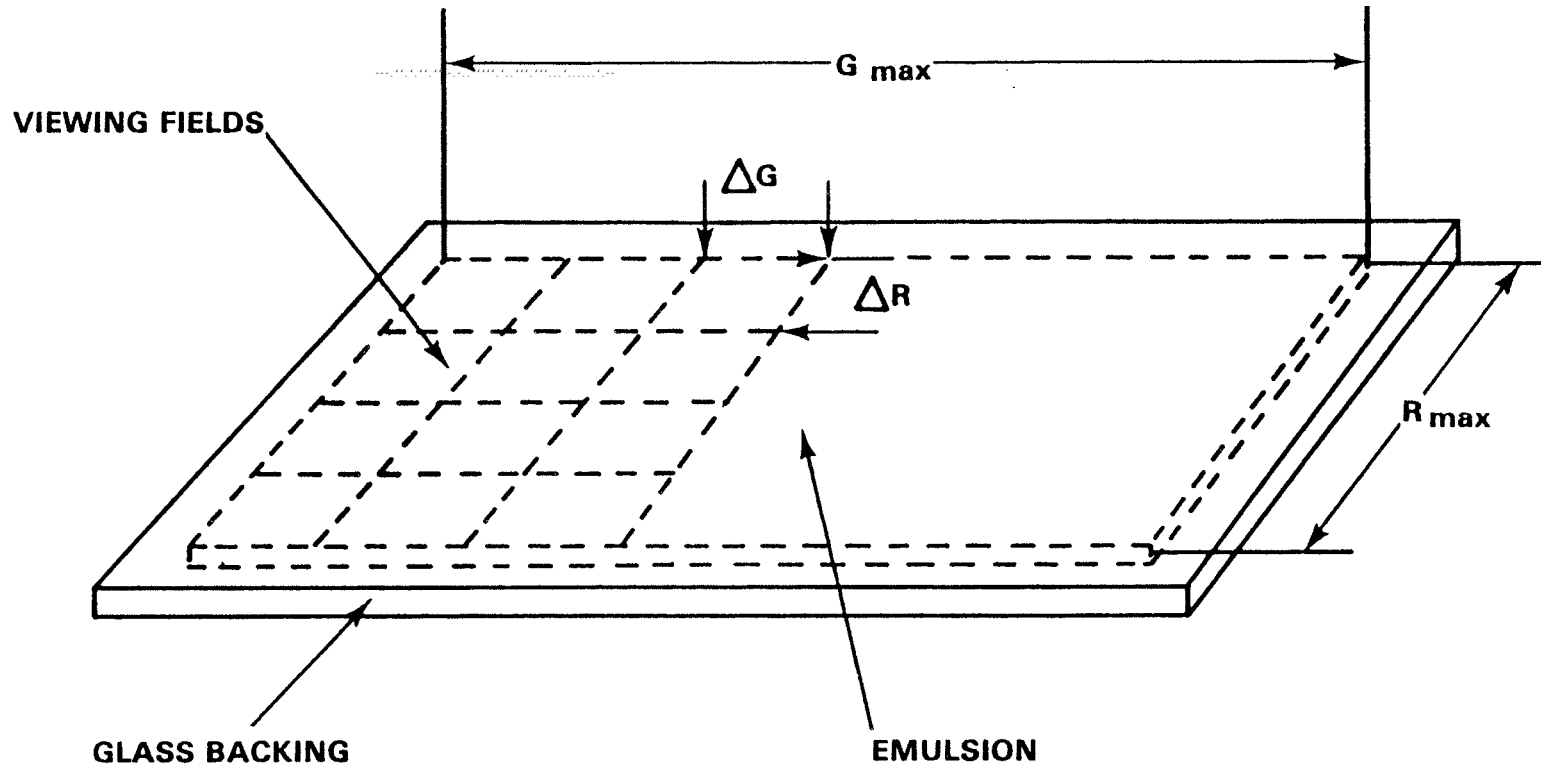
FIG. 6 Maximum Traverse Dimensions, G_{max} and R_{max} , Together with the Field Dimensions, \Delta G and \Delta R , Define the Number of NRE Scanning Fields Available for ESP Operation
