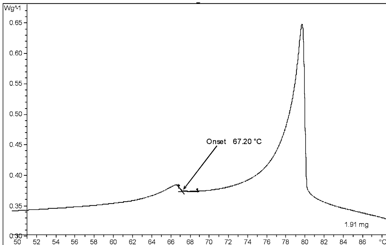
FIG. 1 Cooling Curve for M-24
