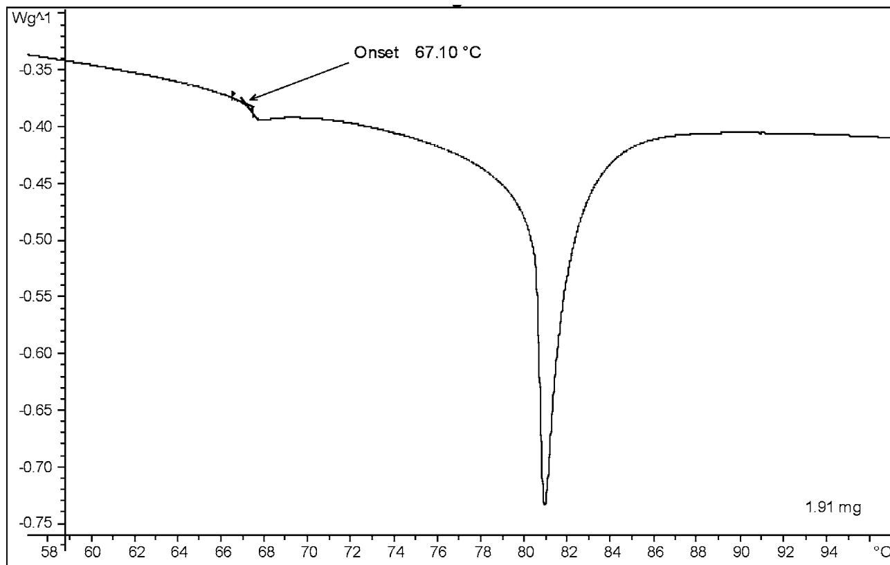
FIG. 2 Heating Curve for M-24
