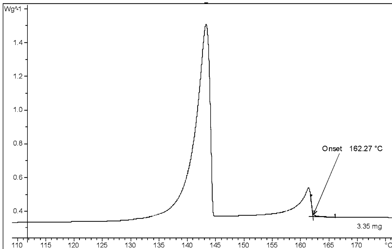
FIG. 5 Cooling Curve for BCH-52
