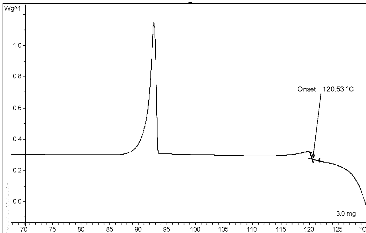
FIG. 3 Cooling Curve for HP-53
