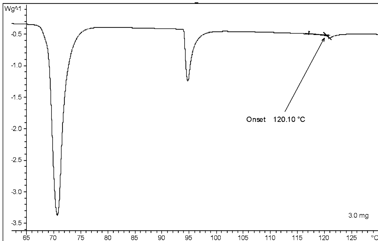
FIG. 4 Heating Curve for HP-53
