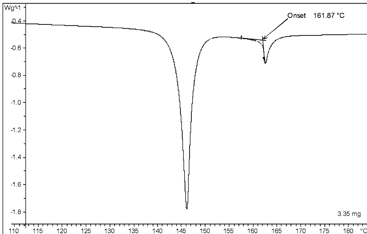
FIG. 6 Heating Curve for BCH-52
