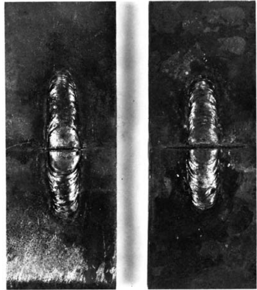
FIG. 15 Typical Examples of No-Break Performance in Drop-Weight Specimens. Fracture Does Not Reach Edge
