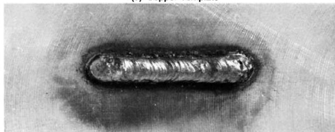
(c) Crack-Starter Weld
