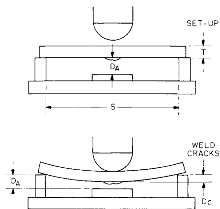
FIG. 11 Drop-Weight Test Method
