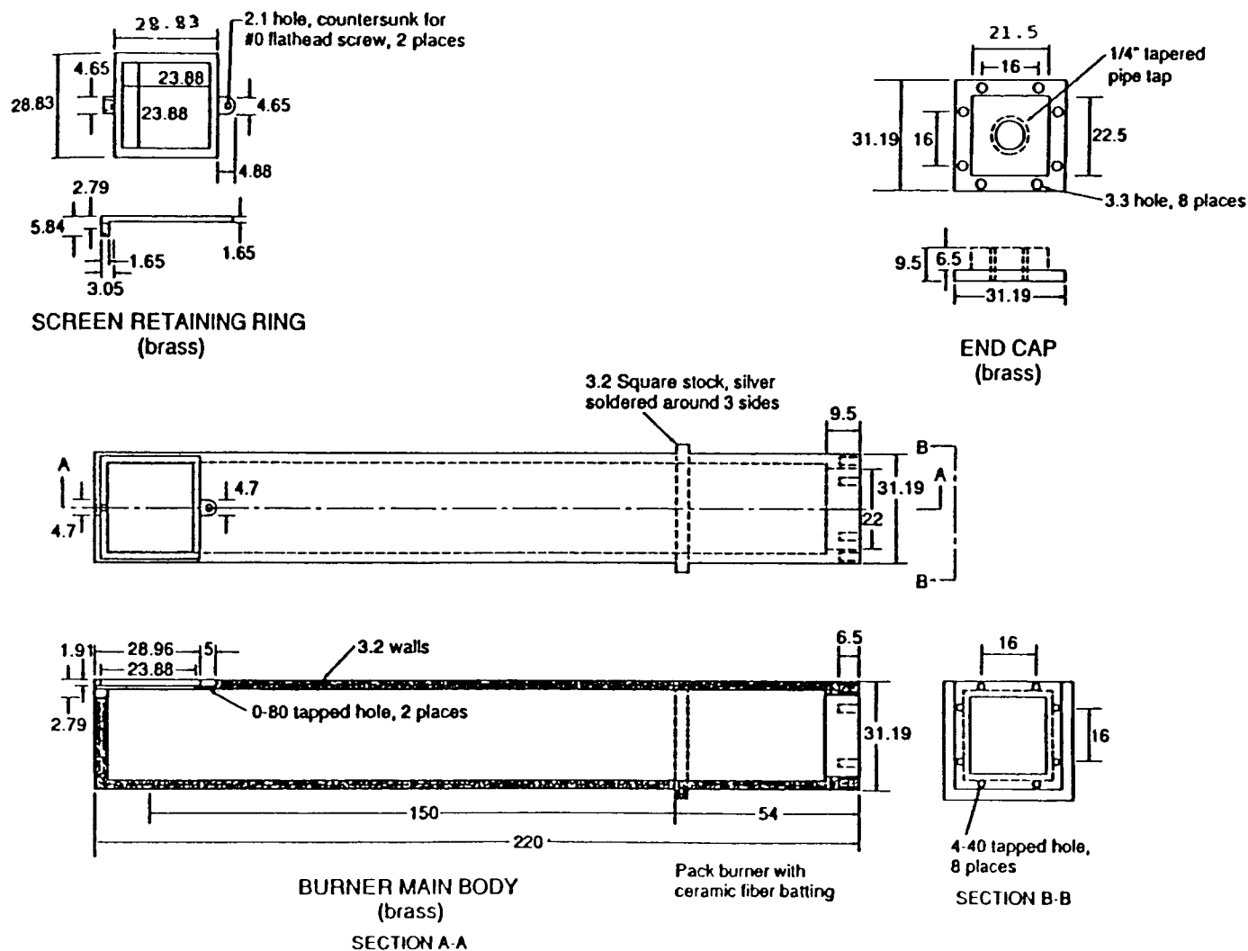
FIG. 5 Calibration Burner
