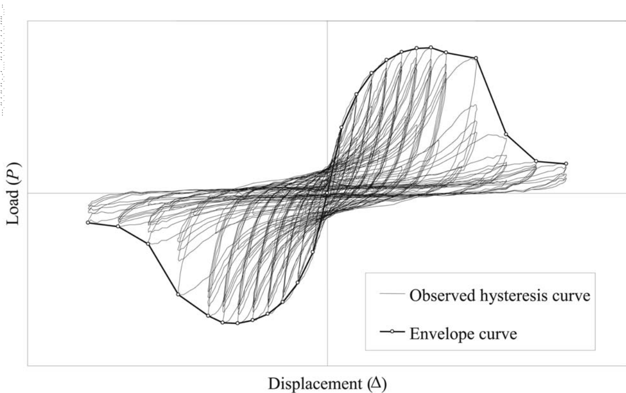
FIG. 2 Examples of Observed Hysteresis Curve and Envelope Curves for Test Method A
