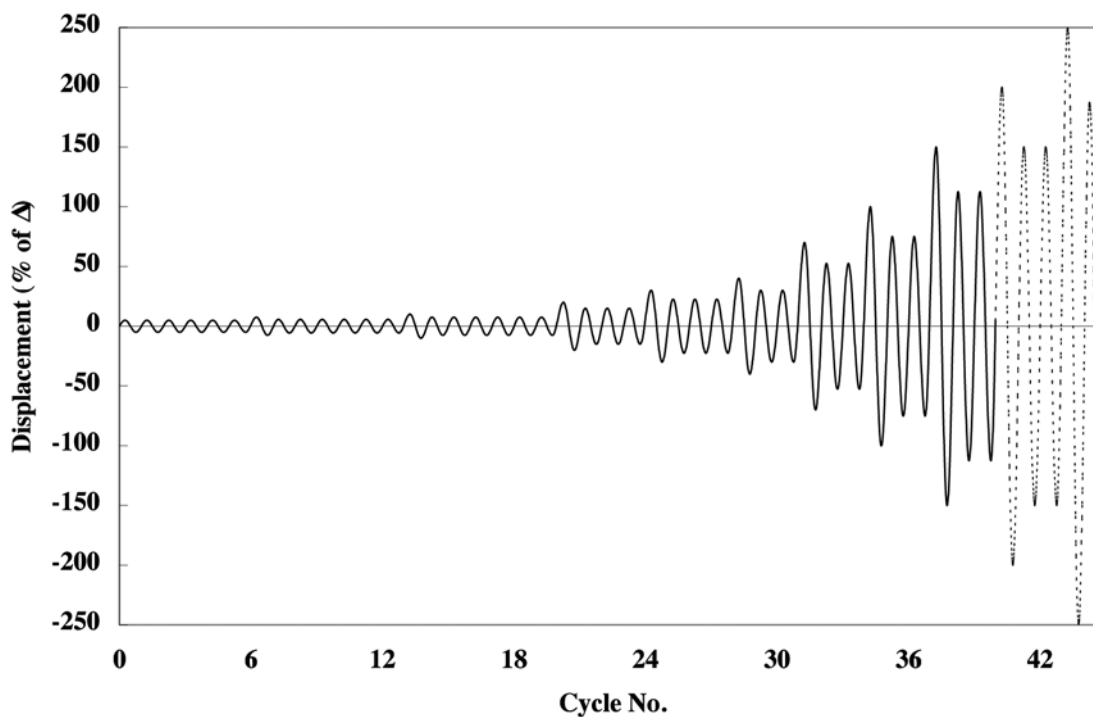
FIG. 9 Cyclic Displacement Pattern (Test Method C)
