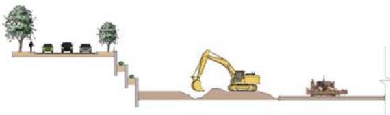
FIG. X2.5 Closed – Detour Traffic Total I-94 Reconstruction
