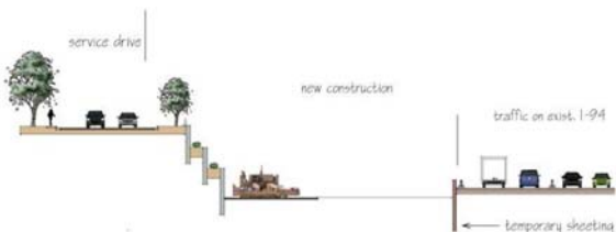
FIG. X2.6 Maintaining Traffic on I-94 Partial I-94 Construction
