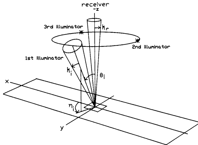
FIG. 4 Circumferential Configuration
