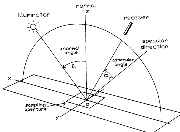
FIG. 1 Uniplanar Configuration
