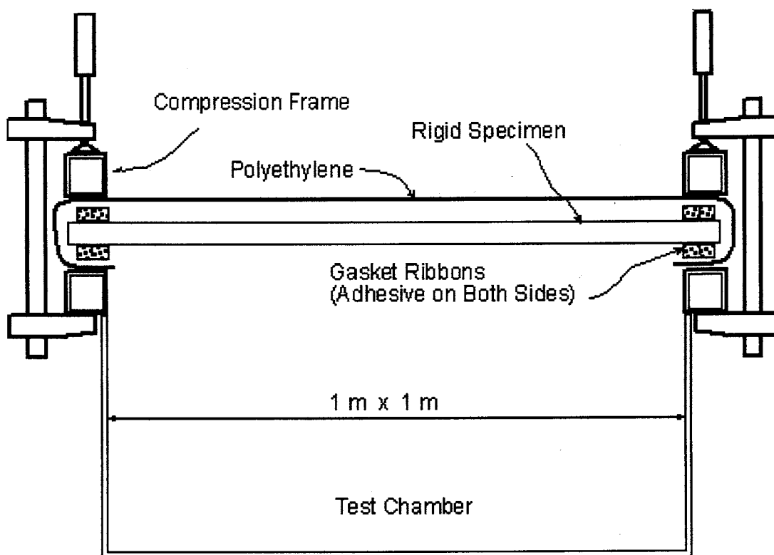
FIG. 5 Rigid Panel-Type Specimen Test Set-up
