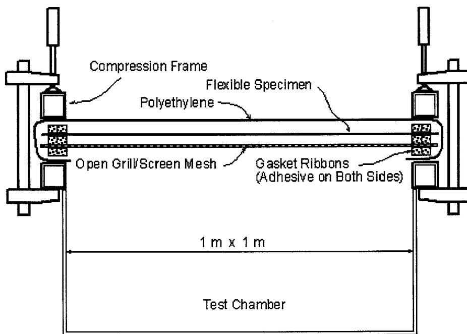
FIG. 2 Flexible Sheet Test Specimen
