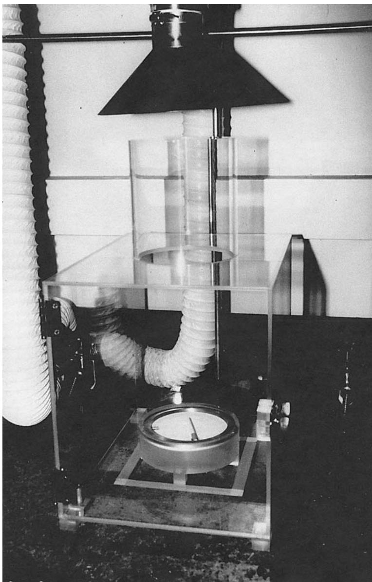
FIG. 1 Photograph of Test Chamber and Filter Paper Holder
