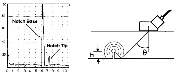
FIG. 21 Example of Second Half-V Path Time of Flight Standardization
