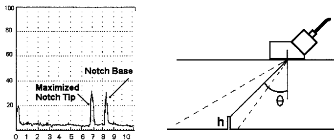
FIG. 19 Example of First Half-V Path Time of Flight (TOF) Standardization
