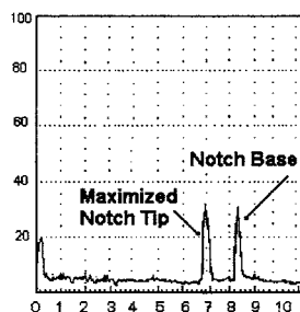
FIG. 19 Example of First Half-V Path Time of Flight (TOF) Standardization
