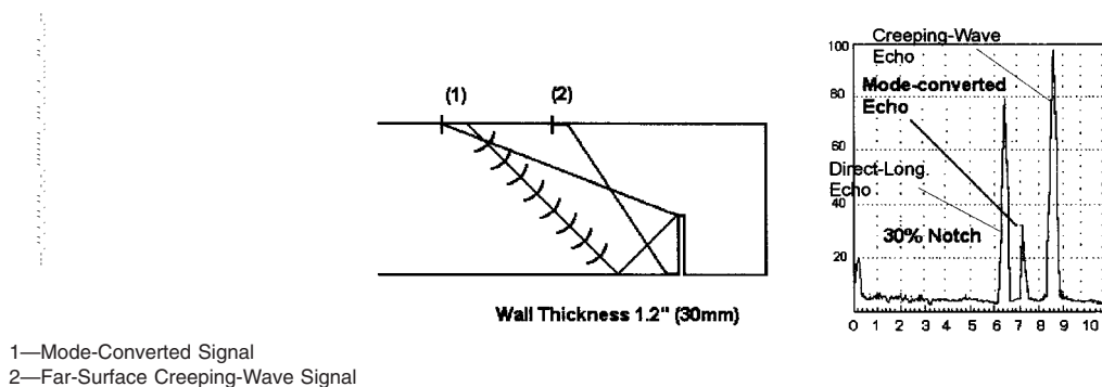
FIG. 4 Search Unit Index Point Position
