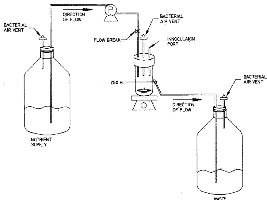
FIG. 1 Rotating Disc Reactor System
