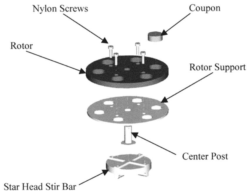
FIG. 2 Rotor Assembly
