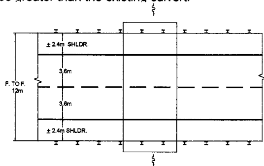
Existing Roadway and Box Culvert
