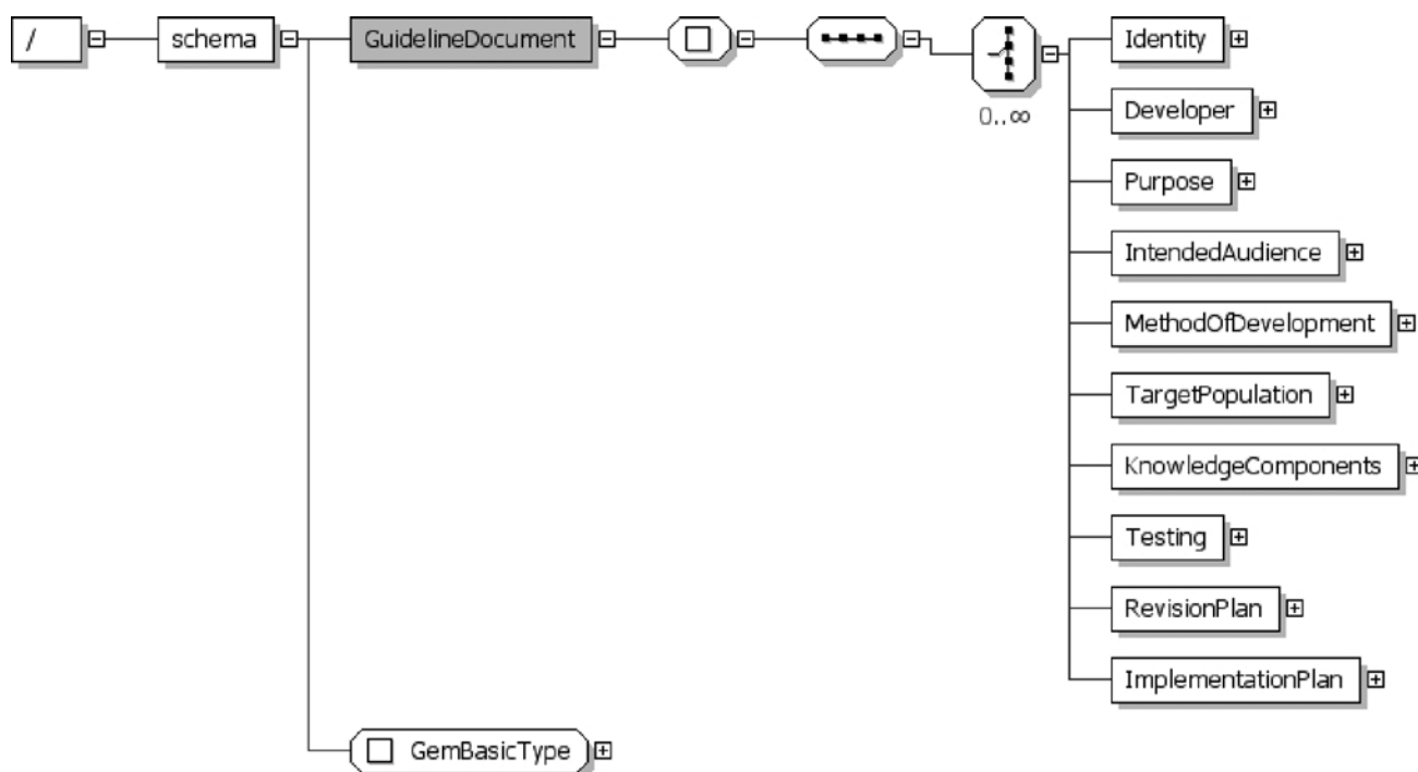
FIG. 1 Top Level of the GEM II Schema
