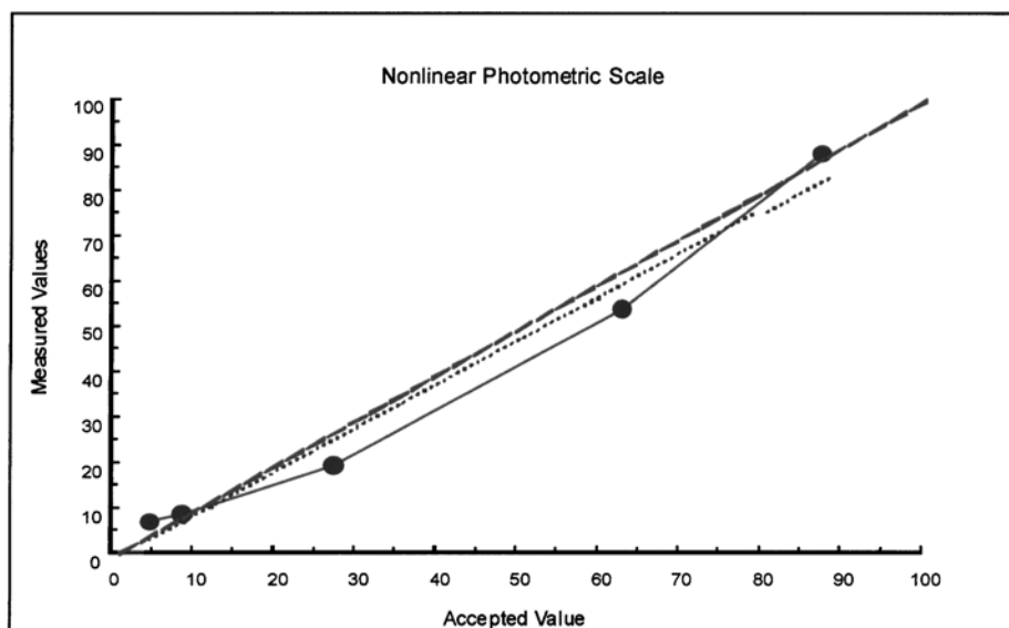
FIG. 2 Nonlinear Photometric Scale
