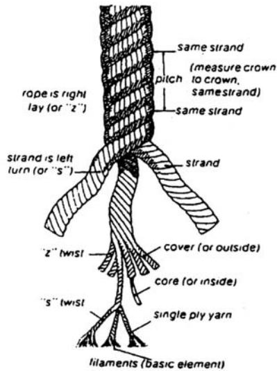
Three-strand rope components
