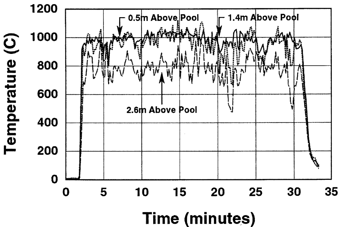
NOTE—The test item was 1 m above the pool. FIG. 12 Temperature Time Histories of Thermocouples in the Fire Near a Test Item
