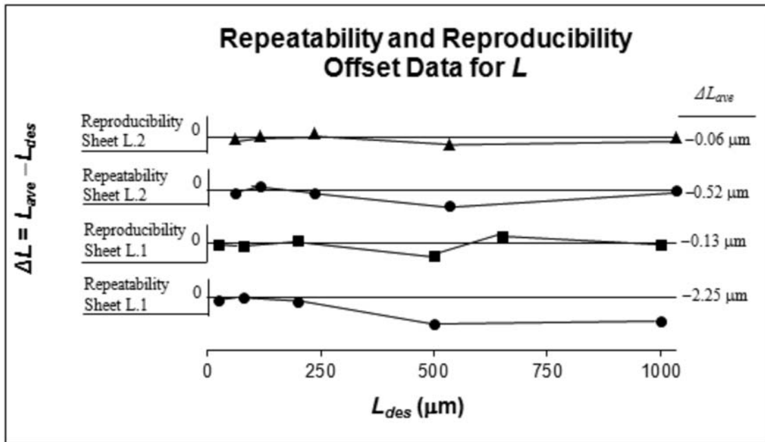
FIG. 9 \Delta L Plotted versus L_{des}
