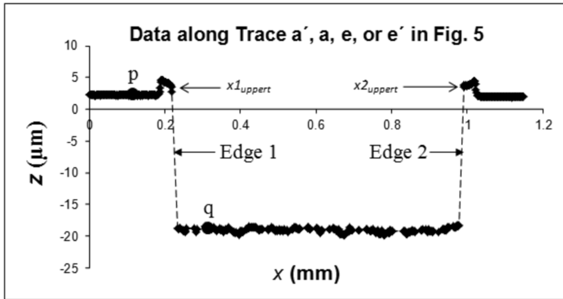
NOTE—Data points are missing along and near Edges 1 and 2. FIG. 6 2-D Data Trace Used to Find x1_{upper} , x2_{upper} , n1_t , and n2_t
