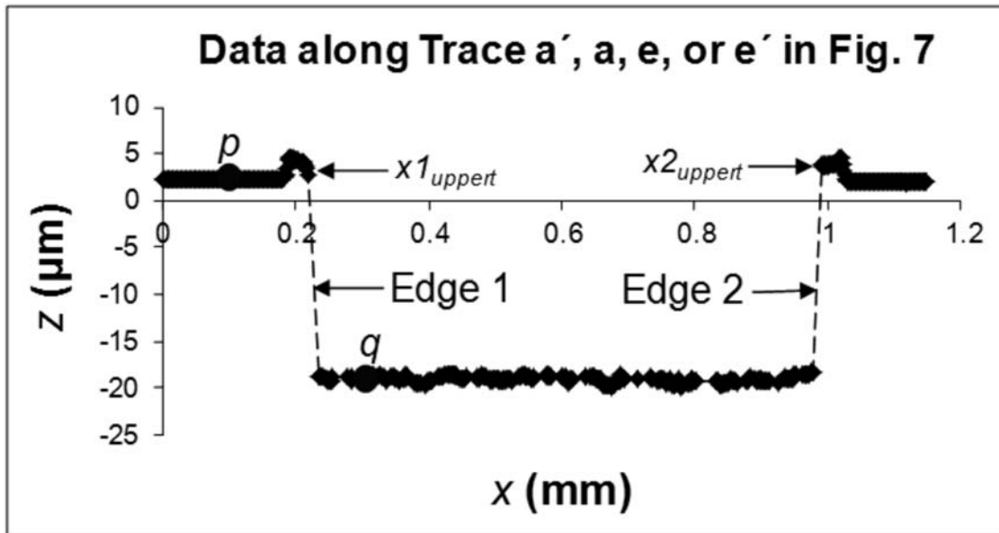
NOTE—Data points are missing along and near Edges 1 and 2. FIG. 8 2-D Data Trace Used to Find x1_{upper} and x2_{upper}
