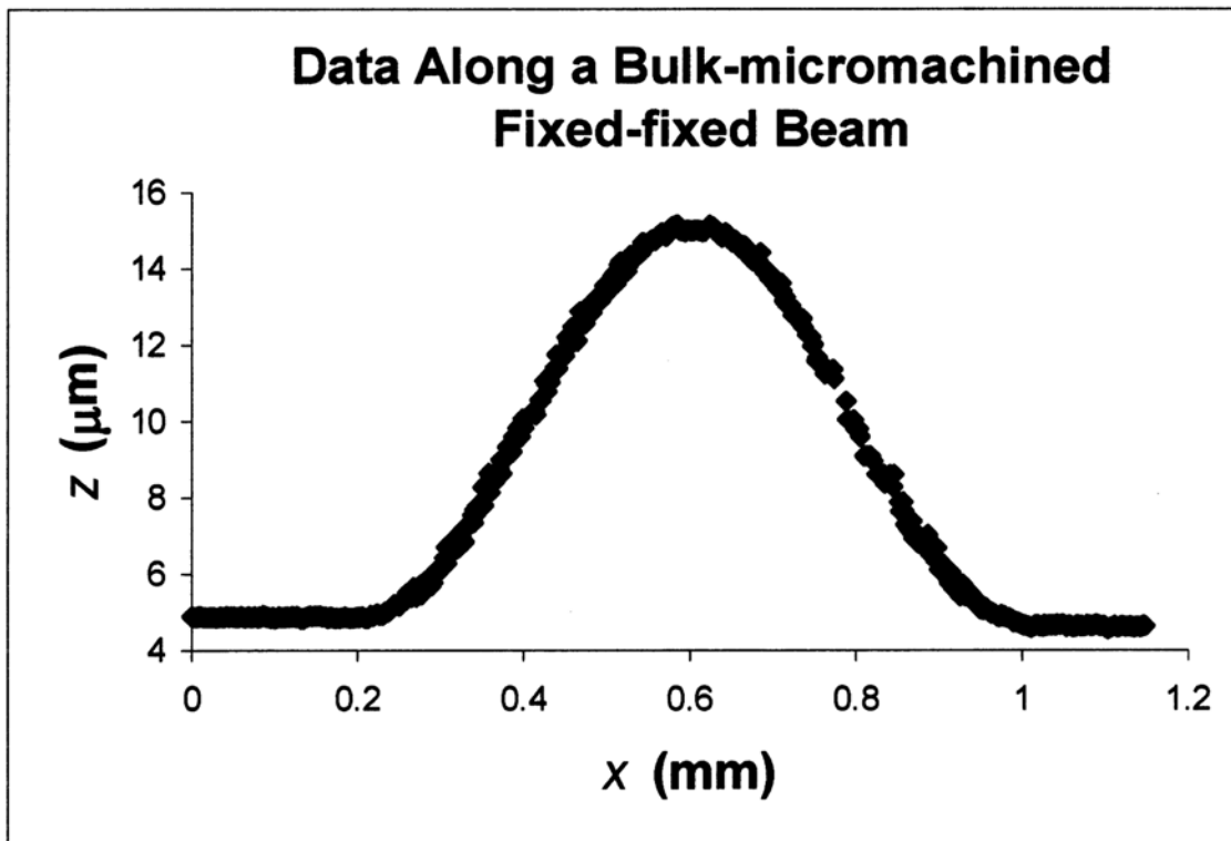
NOTE 1—This is a 2-D data trace ( b , c , or d ) along a fixed-fixed beam similar to that shown in Fig. 7. NOTE 2—Some data points are missing along this trace.
