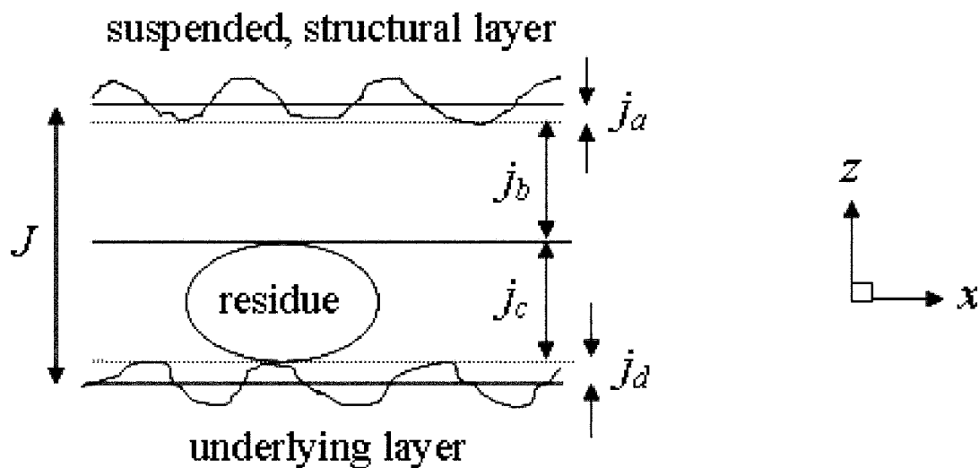
NOTE—This view is along the length of the fixed-fixed beam where it has adhered to the top of the underlying layer. FIG. X1.3 Component Parts of J in Fig. X1.1
