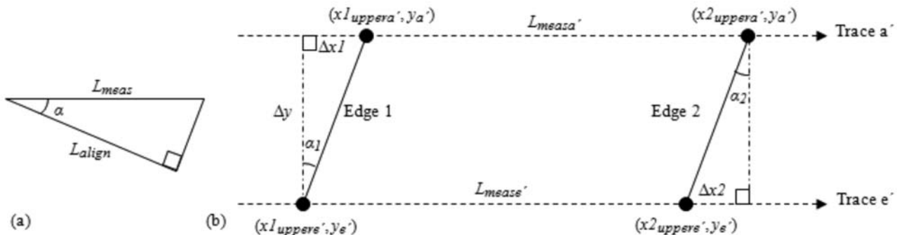
FIG. 11 Drawings Used to Determine a) the Misalignment Angle, \alpha , and b) \Delta x_1 and \Delta x_2
