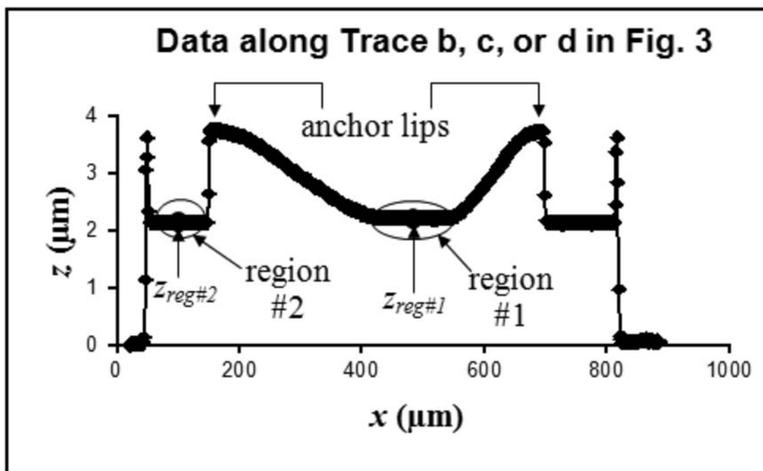
NOTE—This is an example of stiction. FIG. X1.2 2-D Data Trace of Fixed-Fixed Beam in Fig. X1.1
