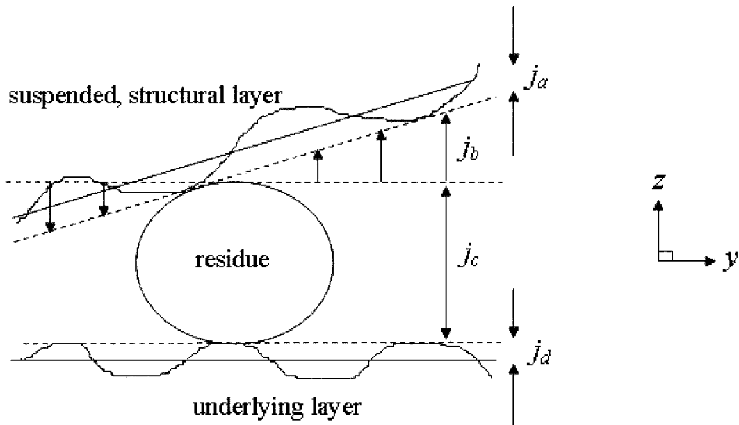
NOTE—This view is along the width of the fixed-fixed beam. FIG. X1.4 Component Parts of J in Fig. X1.1 and Fig. X1.3
