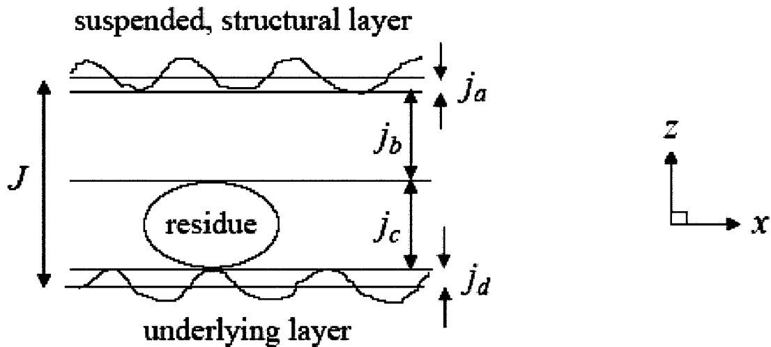
NOTE—This view is along the length of the cantilever where it has adhered to the top of the underlying layer. FIG. X1.3 Component Parts of J in Fig. X1.1
