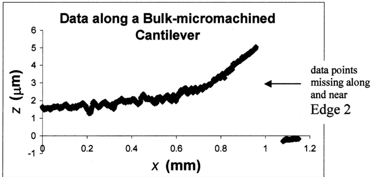
NOTE—This is a 2-D data trace ( b , c , or d ) along a cantilever similar to that shown in Fig. 7. FIG. 9 2-D Data Trace Used in Strain Gradient Calculation
