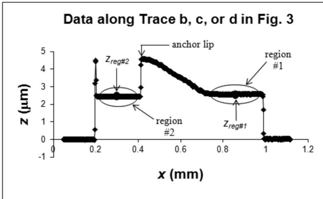
NOTE—This is an example of stiction. FIG. X1.2 2-D Data Trace of Cantilever in Fig. X1.1
