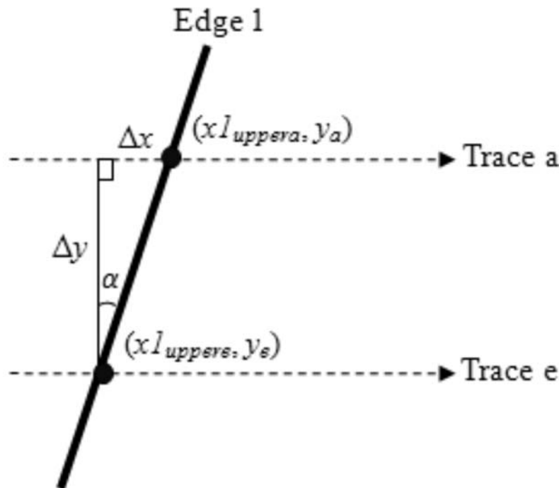
FIG. 10 Sketch Depicting the Misalignment Angle, \alpha
