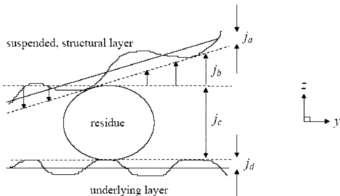
NOTE—This view is along the width of the cantilever. FIG. X1.4 Component Parts of J in Fig. X1.1 and Fig. X1.3
