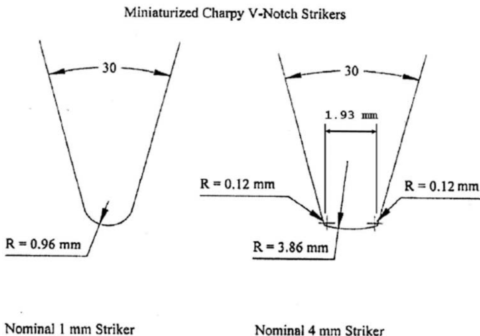
FIG. 1 Scaled 8 mm and 2 mm Strikers for Use in Miniaturized Charpy Impact Test
