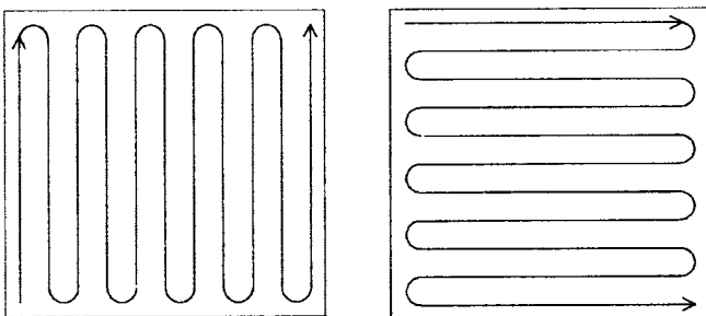
FIG. 6 Scan patterns for the first and second scans differ in orientation by 90°. The measured intensities are L_{Ink}(1) and L_{Ink}(2) , respectively. The difference in the measured intensity levels is used to determine the adequacy of the scan line density and the measurement reproducibility.
