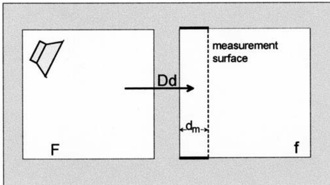
A sketch showing a measurement surface used to sample the partition wall. The dark lines indicate the portion of flanking surfaces that are contained in the measurement volume. Using the indicated measurement surface, and without the shielding of any surfaces, the following paths will be measured D_d , F_d and a fraction of D_j and F_j .
