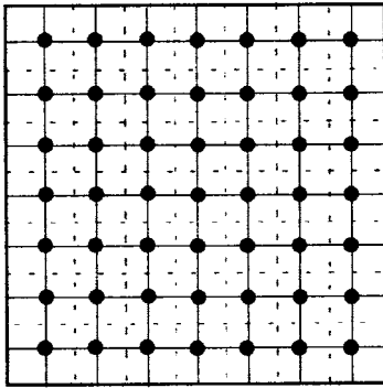
FIG. 5 Typical construction of the measurement grid for discrete point measurements. The dots indicate the sampling locations while the dashed lines define the area sampled by each point.
