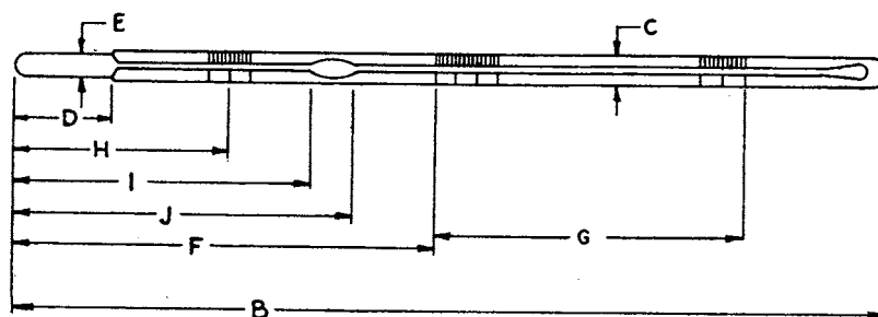
FIG. 1 Total Immersion Thermometer with Auxiliary Ice Point
