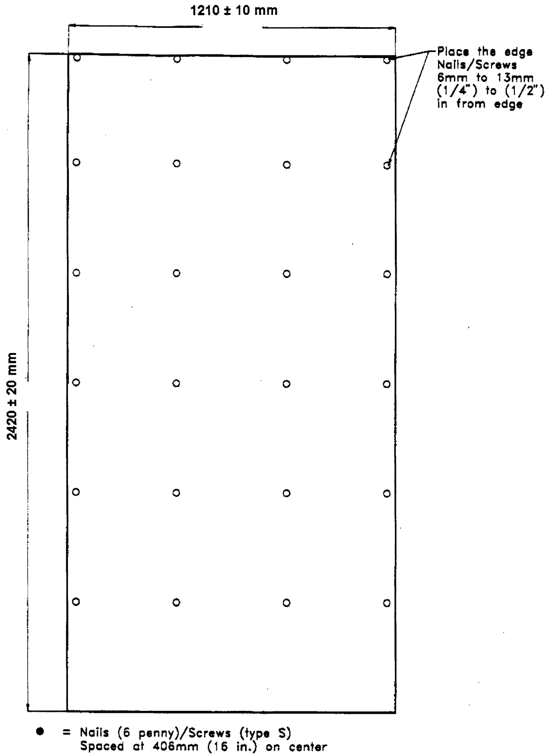
FIG. X2.4 Attachment Details for Thermoplastic Wall Materials
