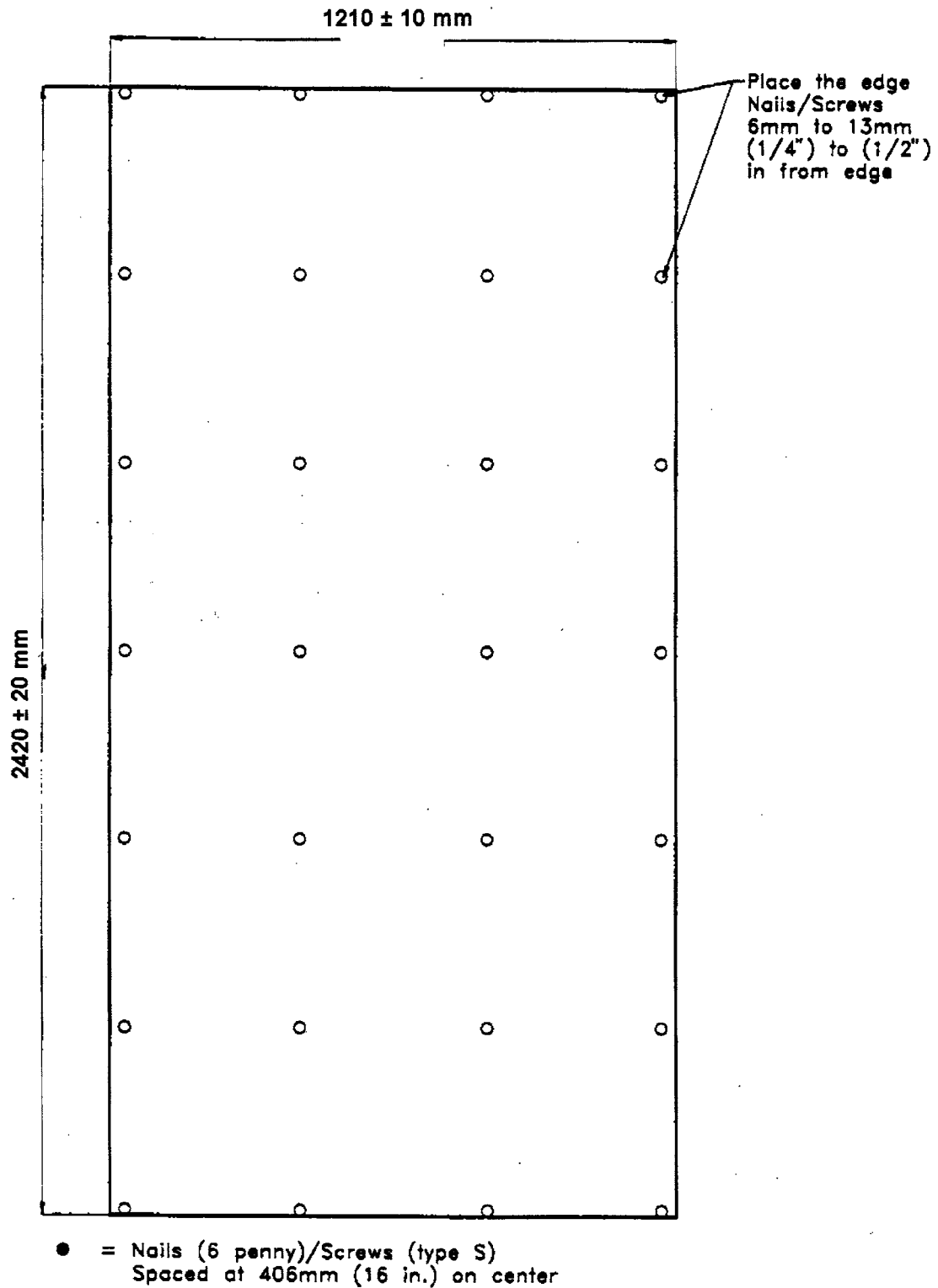
FIG. X2.5 Attachment Details for Ceiling Materials
