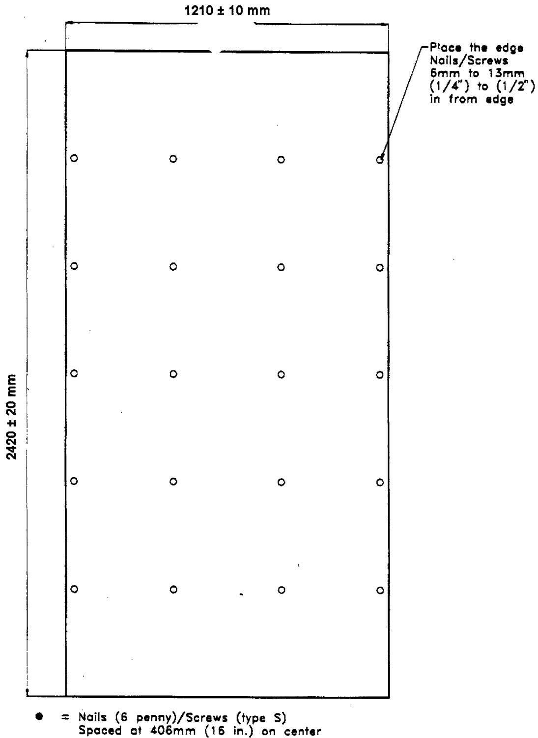
FIG. X2.3 Attachment Details for Rigid Wall Materials
