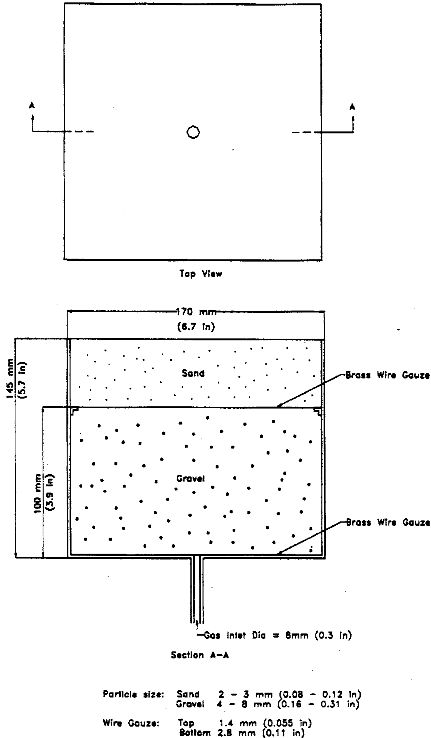
FIG. 1 Gas Burner Ignition Source
