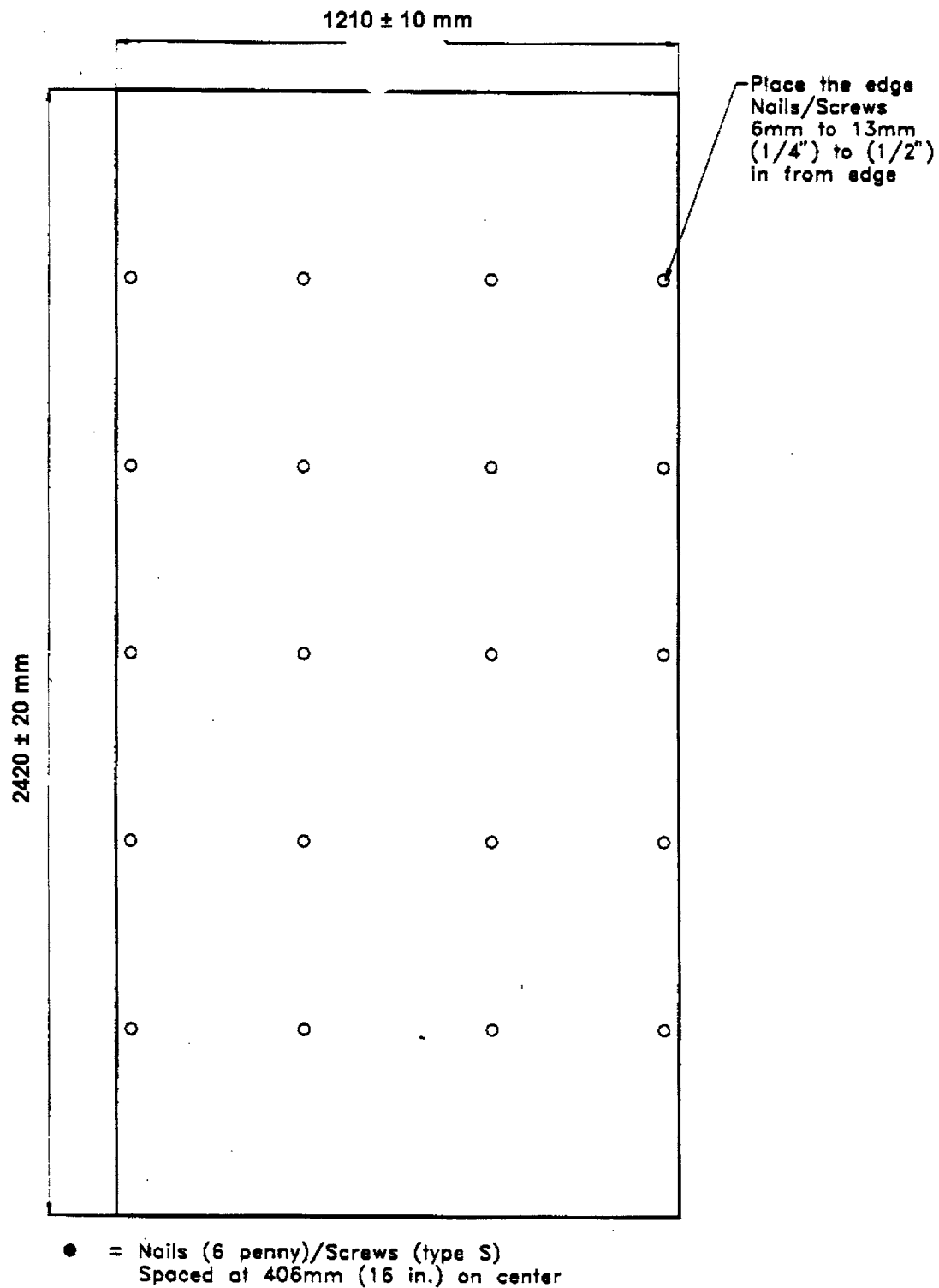
FIG. X2.3 Attachment Details for Rigid Wall Materials
