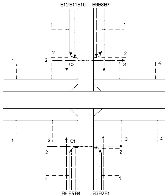
FIG. 9 Scans of the Horizontal Weld into a Cut Out
