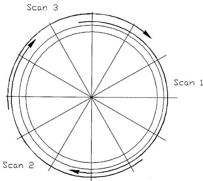
FIG. 4 Scanning Pattern for a Circumferential Weld
