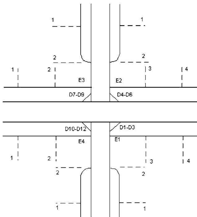
FIG. 10 Nomenclature for Vertical Welds
