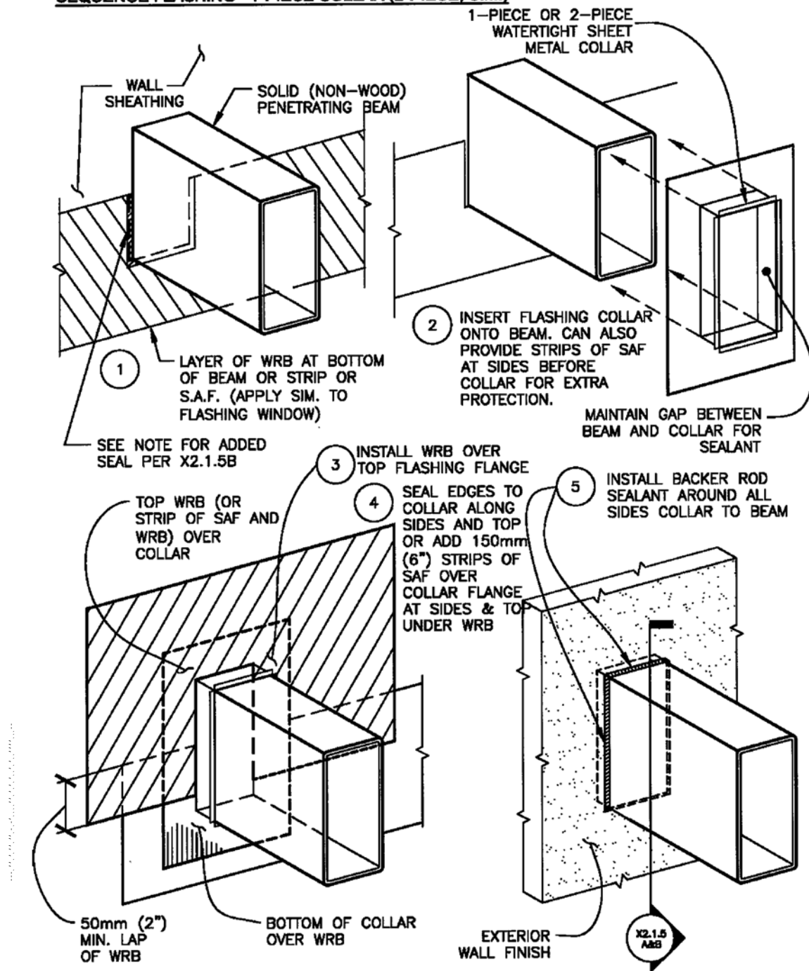
X2.1.5C BEAM PENETRATION FLASHING COLLAR -
