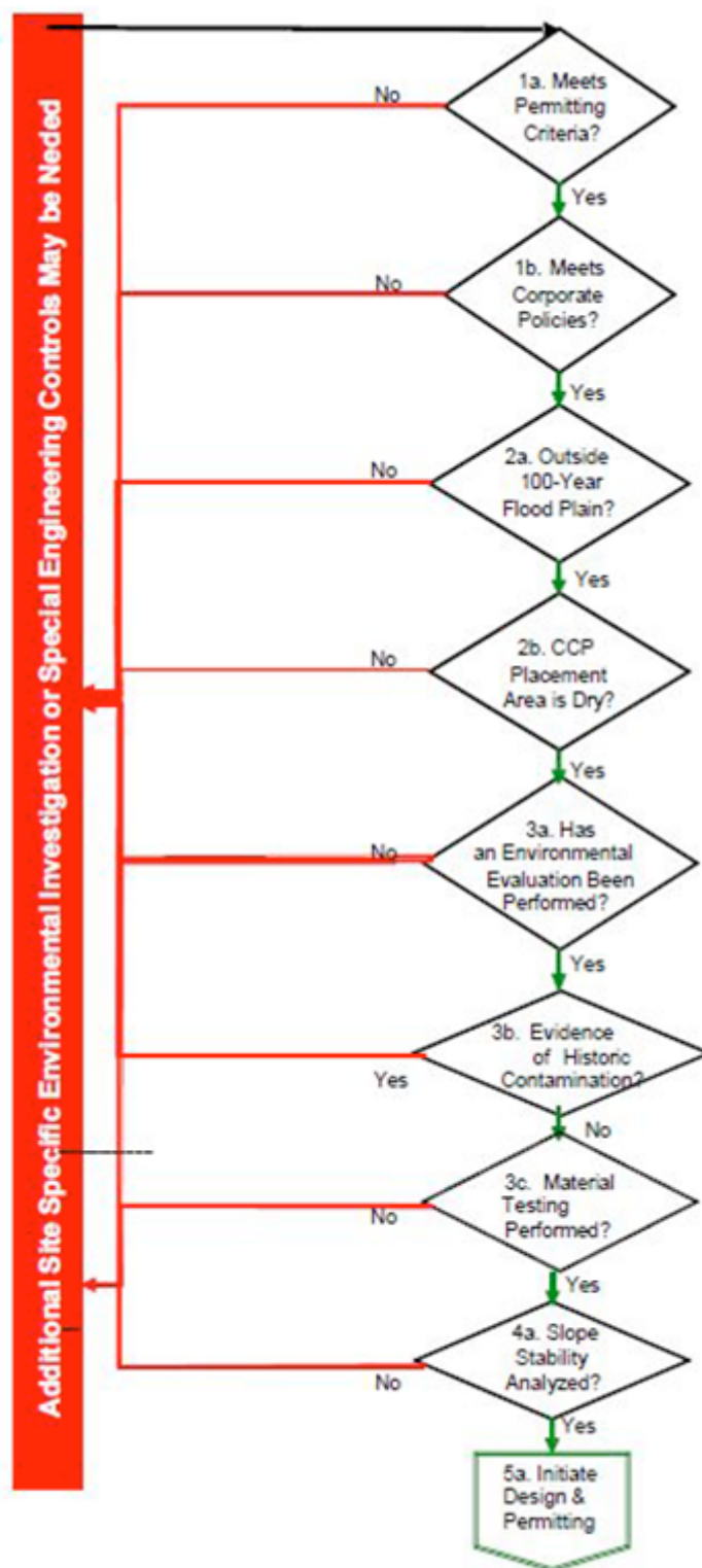
FIG. 1 Environmental Flow Chart CCP Engineered Structural Fills
