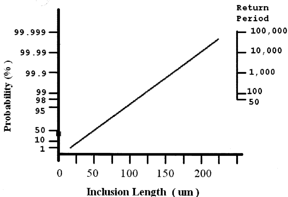
FIG. X1.2 Graphical Representation of the Extreme Value Distribution of Steel Z
