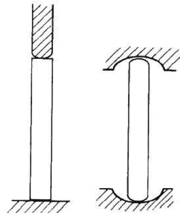
FIG. 2 Suggested Shapes of Specimen's and Push-Rod Ends
