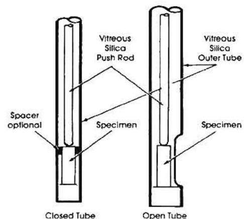
FIG. 1 Common Forms Specimen Holders
