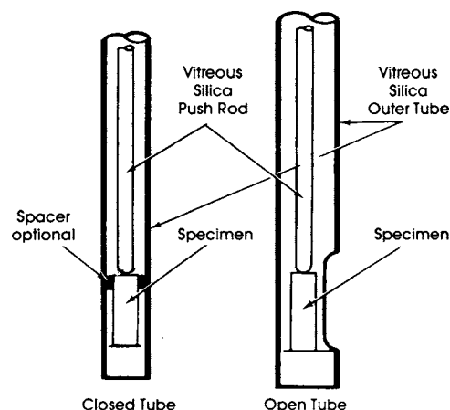
FIG. 1 Common Forms Specimen Holders
