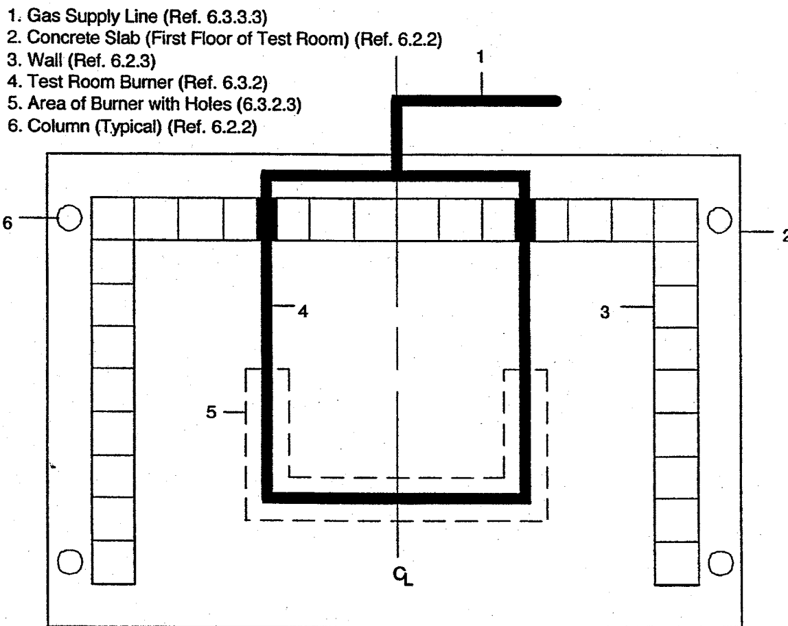
FIG. 1 Plan View of Test Room Burner Positioned in Test Room (See 6.3.2 for Dimensions)
