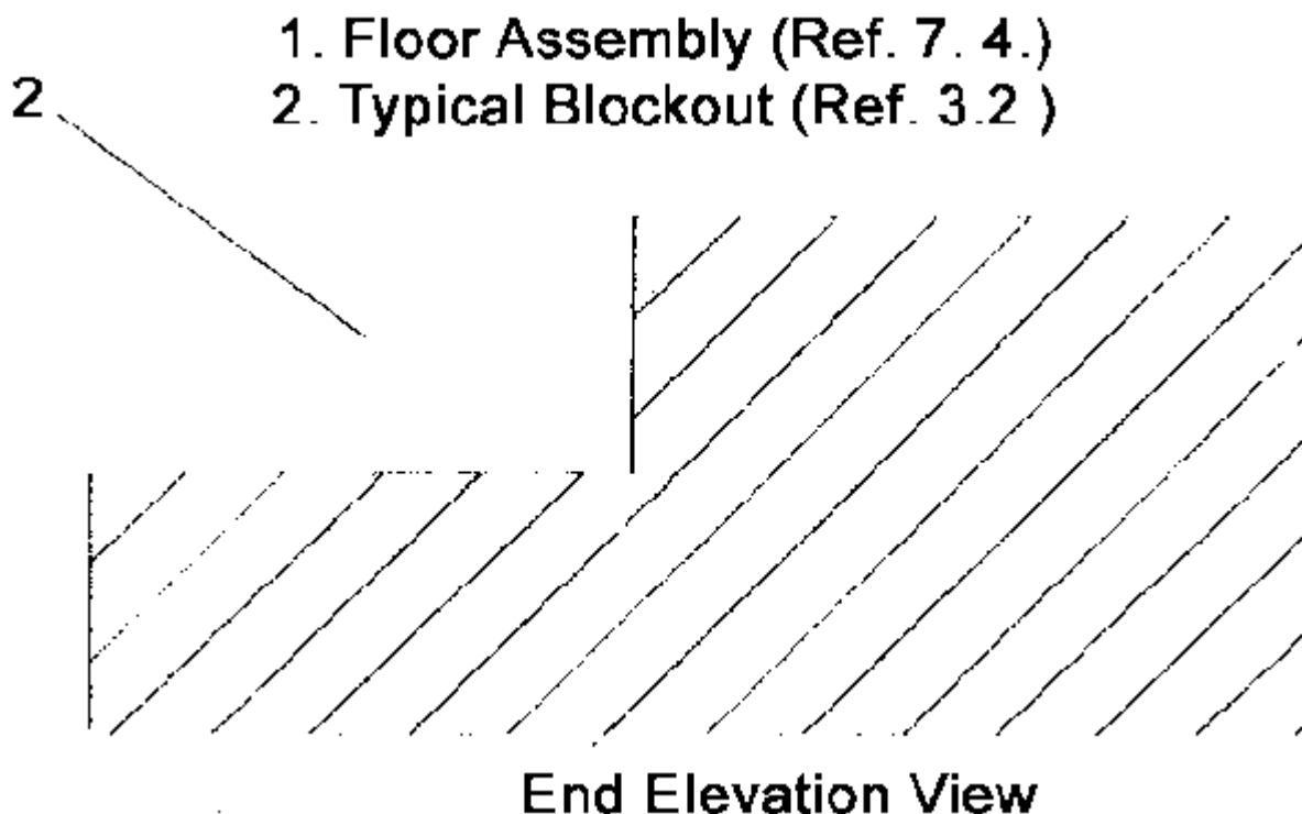
FIG. 13 Typical Blockout (See 12.2.4.3)
