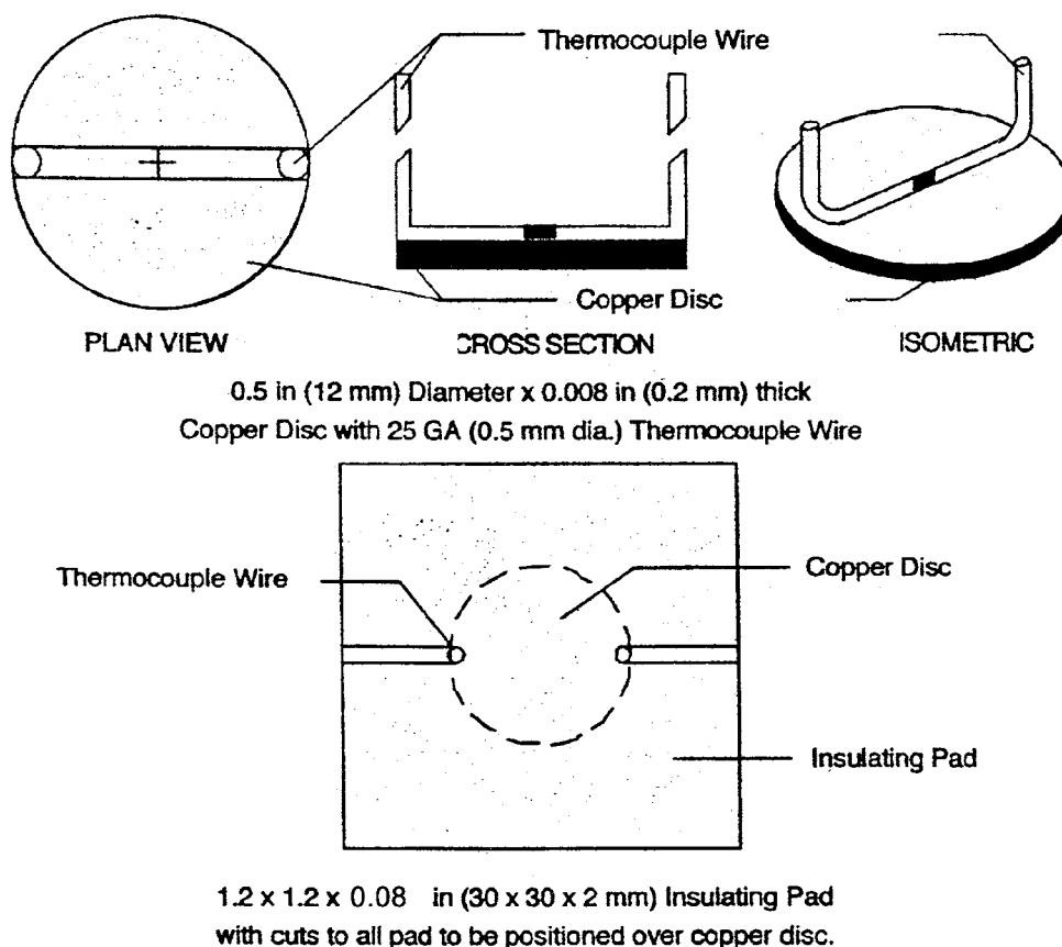
FIG. 4 Typical Copper Thermocouple Disc and Insulating Pipe (See 6.6 and 6.7)
