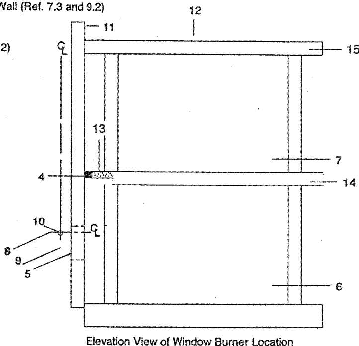
FIG. 2 Plan View of Window Burner and Elevation View of Window Burner Location
