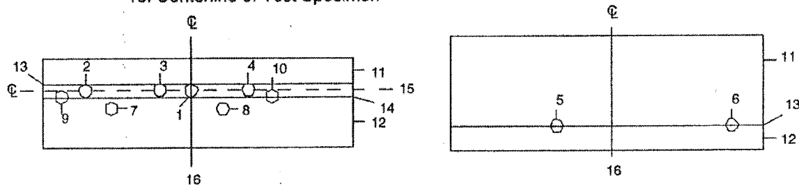
Plan View of Observation Room Floor at Perimeter Joint Treatment
