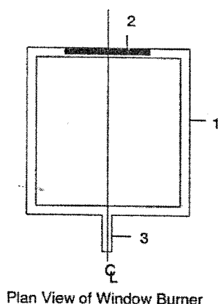
FIG. 2 Plan View of Window Burner and Elevation View of Window Burner Location
