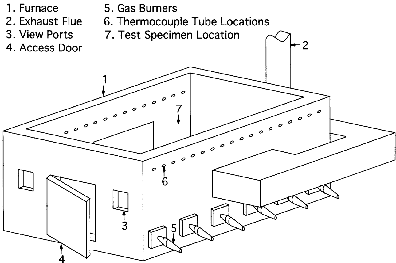
FIG. 3 A Horizontal Furnace
