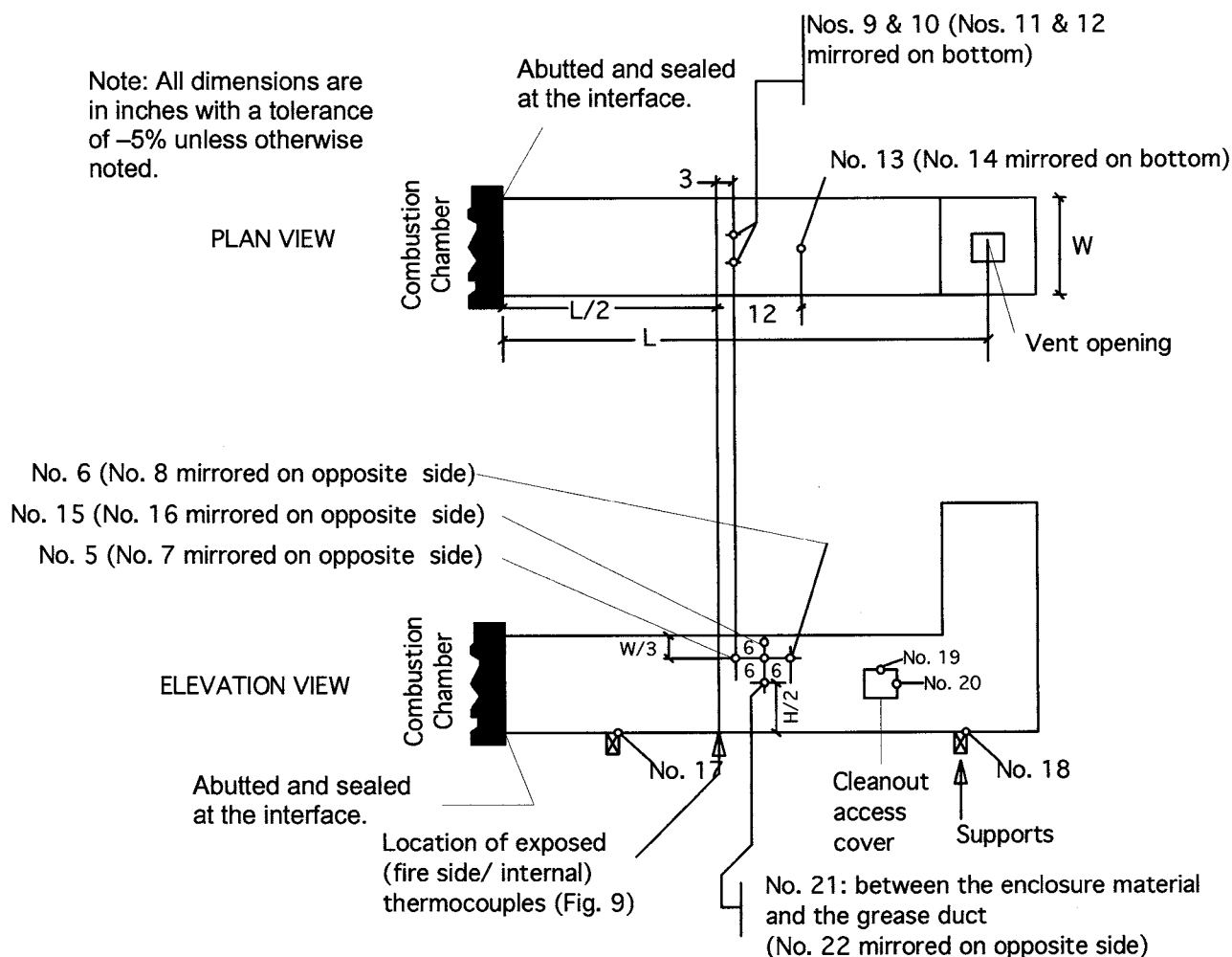
FIG. 10 Unexposed Surface Thermocouple Locations
