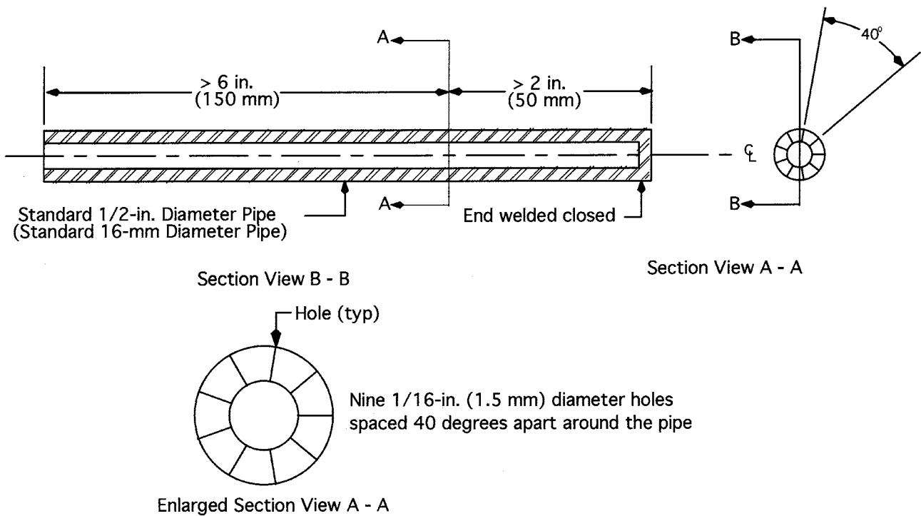
FIG. 5 Tube Sensor
