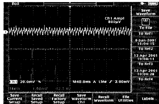
FIG. 4 800 \mu V Signal
