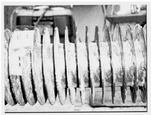
FIG. 7 Sawtooth Wear Pattern
