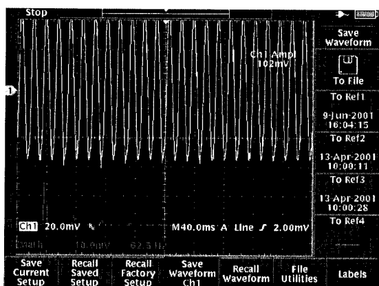
FIG. 8 102 mV Signal
