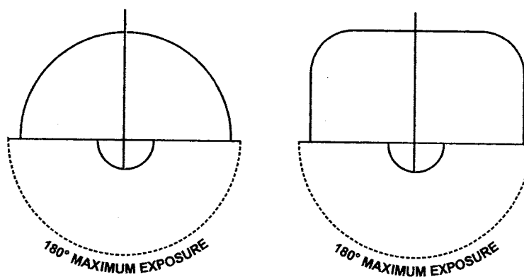
FIG. 6 Portable Grinders
