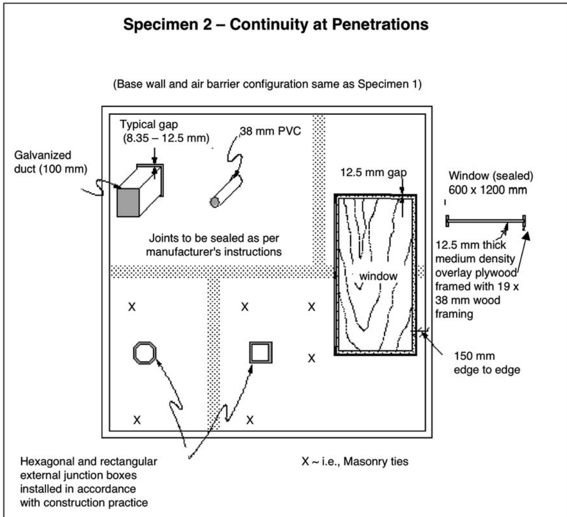
FIG. A1.2 Specimen 2—Continuity at Penetrations
