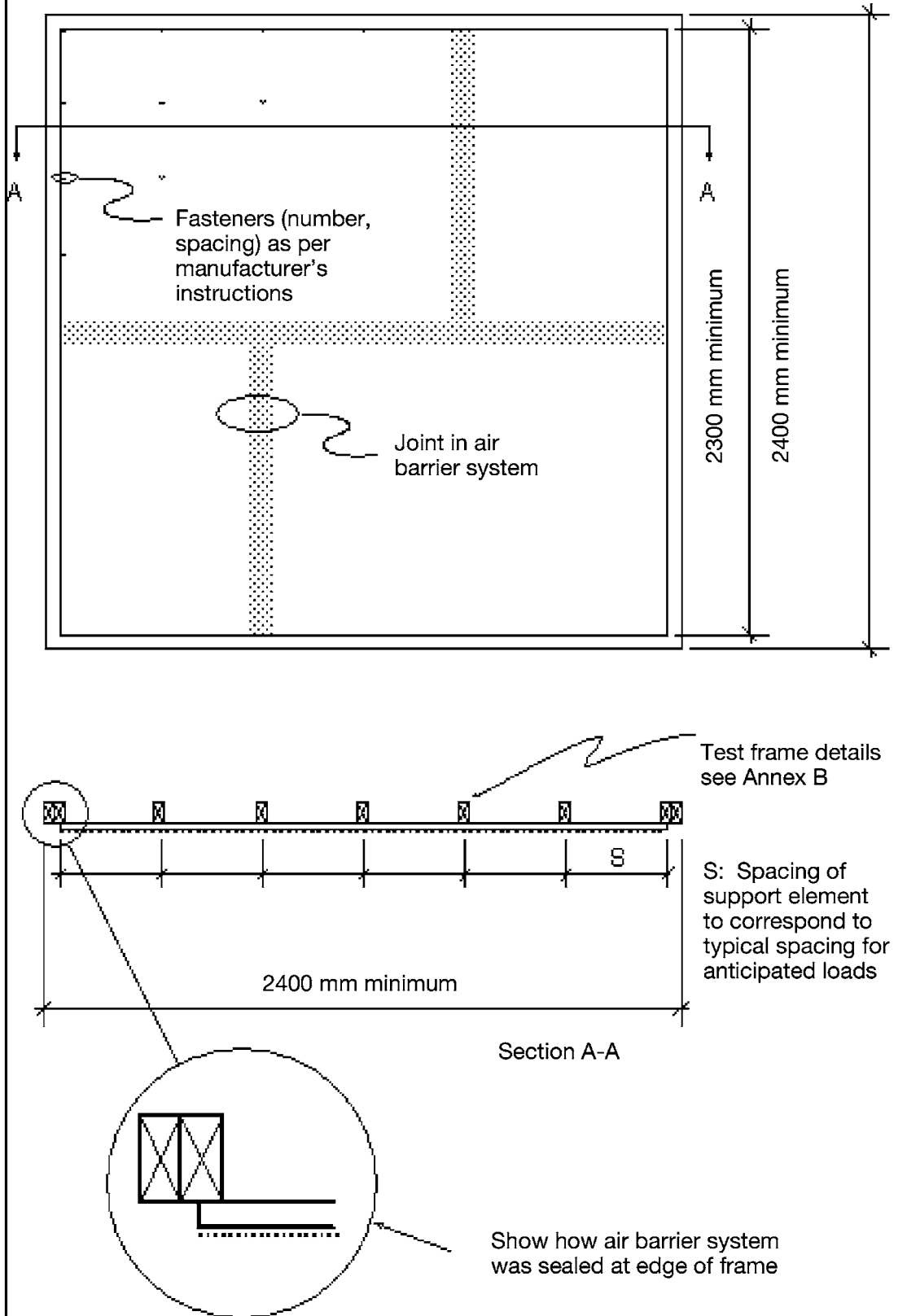
FIG. A1.1 Specimen 1—Opaque Wall
