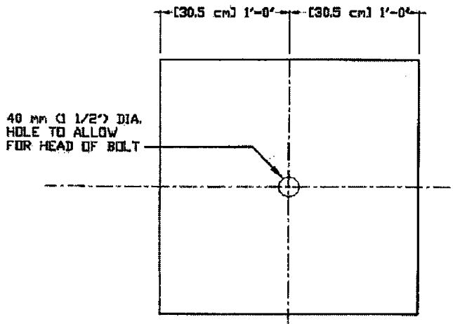
FIG. 2 Bonding panel
