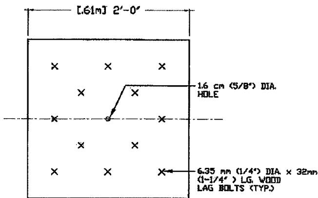
FIG. 3 Bolting Panel
