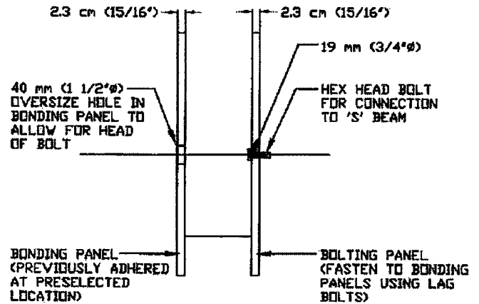
FIG. 4 Plywood Assembly
