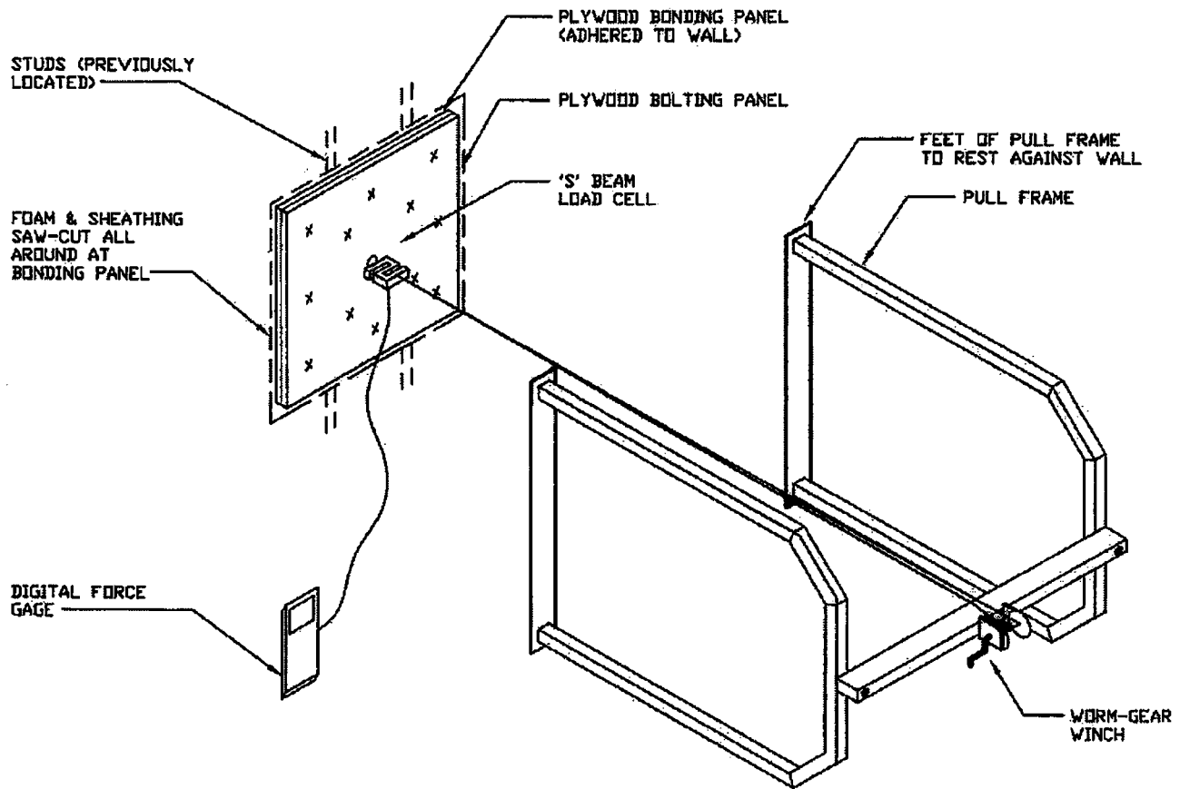
FIG. 6 Test Arrangement Isometric
