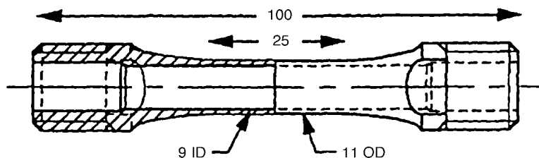
Cylindrical smooth shank TMF tube, Ref. 3.
