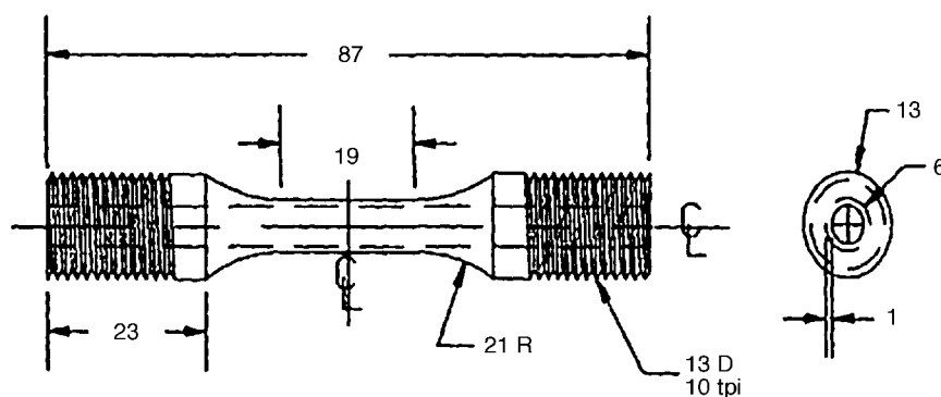
Cylindrical threaded shank TMF tube, Ref. 2.
