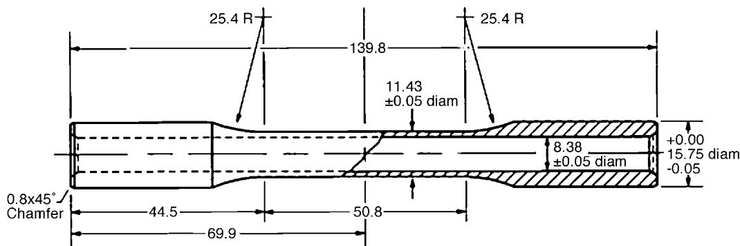
Cylindrical smooth shank TMF tube, Ref. 1.
