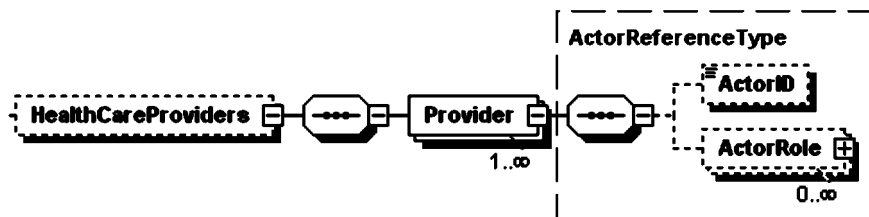
FIG. A2.24 <HealthCareProviders> Data Object
