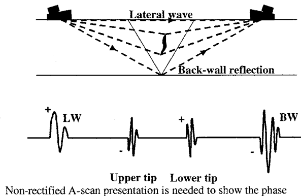
FIG. 1 TOFD Configuration and Signal Origins
