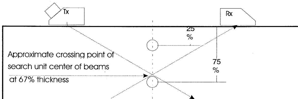
FIG. X1.1 Reference Block for Single TOFD Pair
